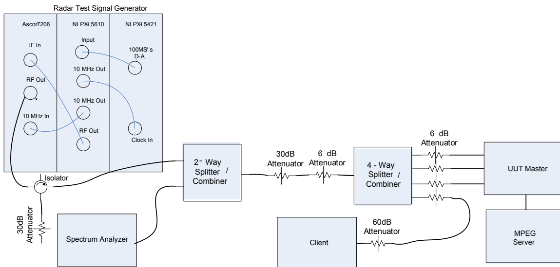
Conducted Setup: Radar Test Waveforms are injected into the Master
