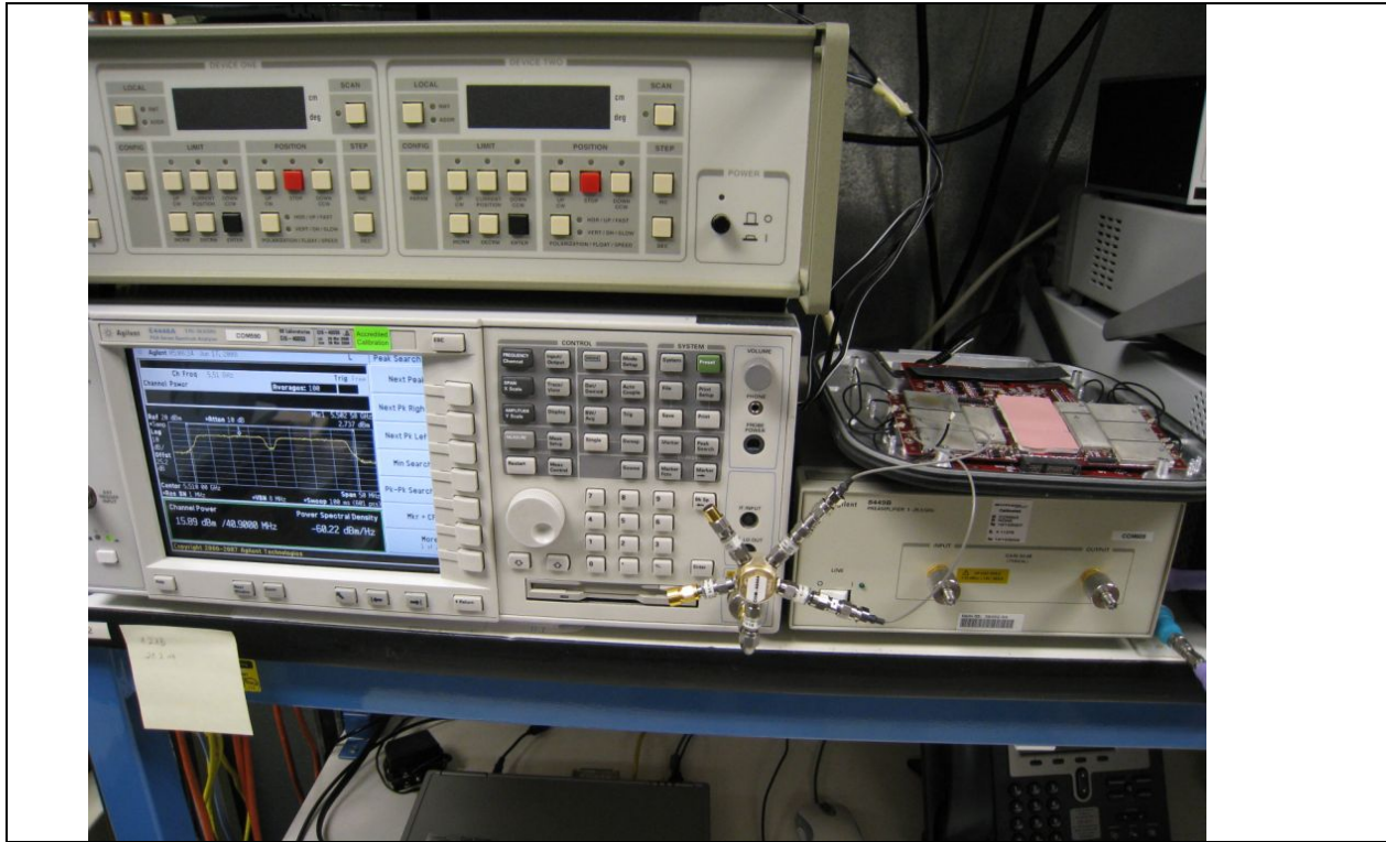
Title: Conducted Test Setup
