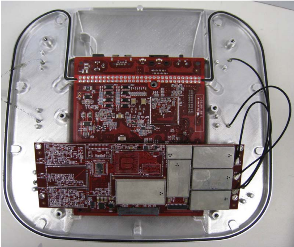
Mother Board
