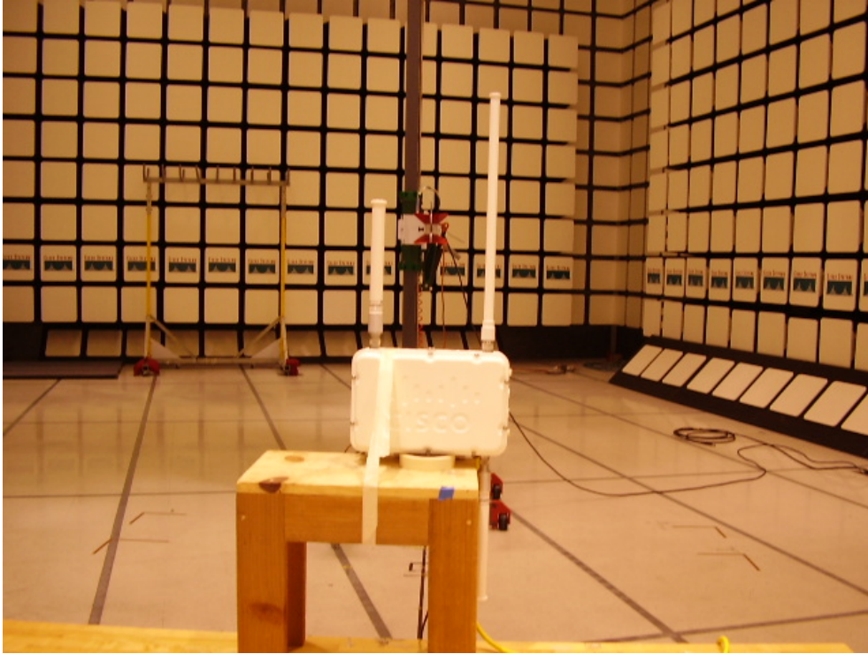
Radiated Emissions, 4.9GHz 17 dBi Sector Antenna, 5GHz 17dBi Sector Antenna with 2.4GHz 8dBi Omni Antenna
