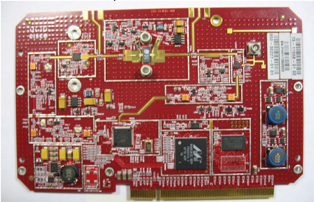
AIR-RM1520-58 Unshielded Top
