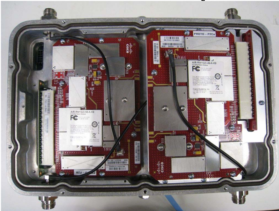
AIR-RM1520-58 Installed in AIR-LAP1524 Series Housing
