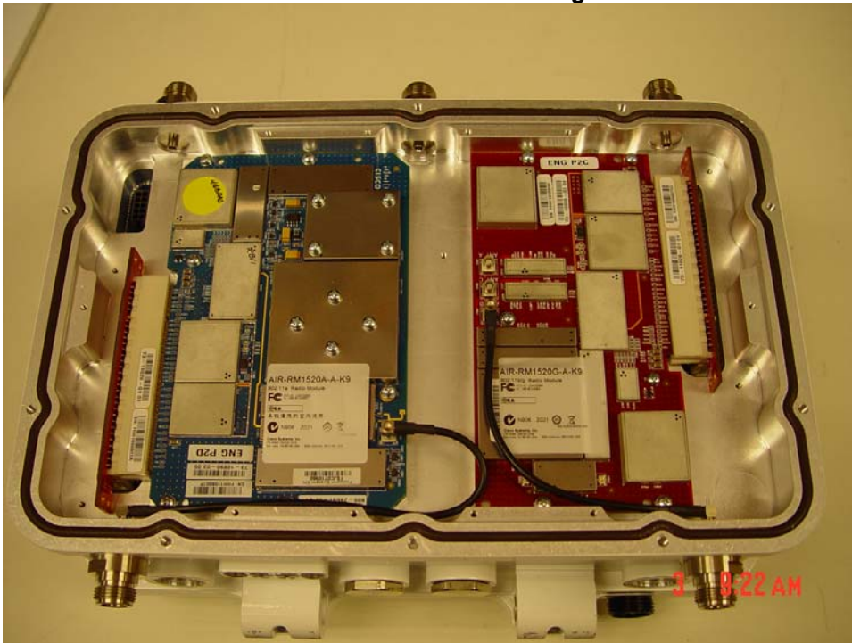
AIR-RM1520G Installed in AIR-LAP1522AG Housing
