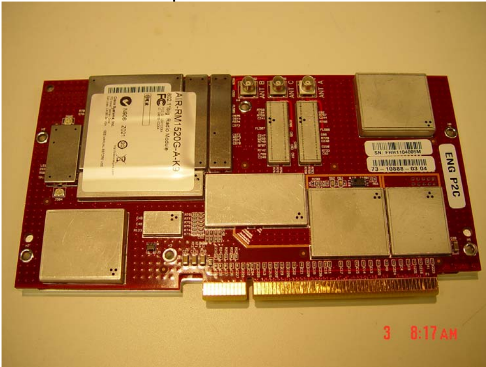
AIR-RM1520G Shielded Top
