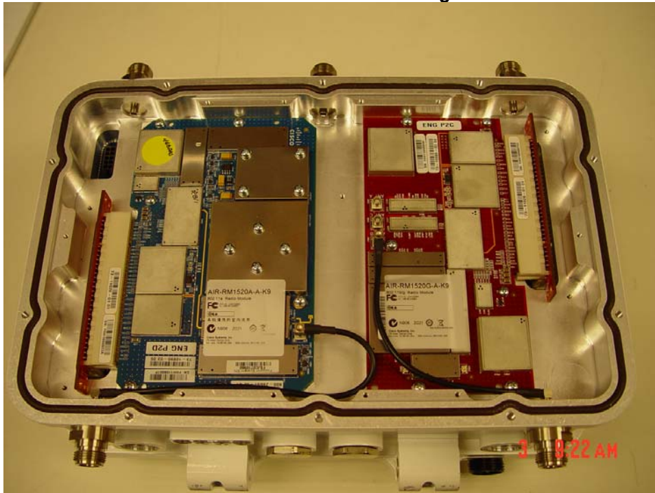
AIR-RM1520A Installed in AIR-LAP1522AG Housing
