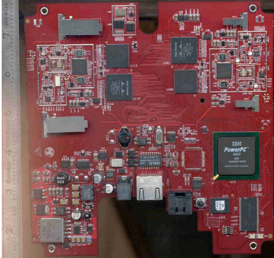
Top with Shields Removed
