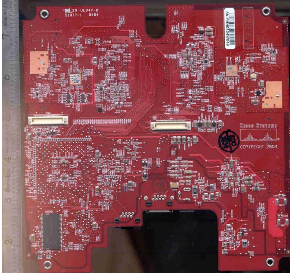
Bottom with Shields Removed
