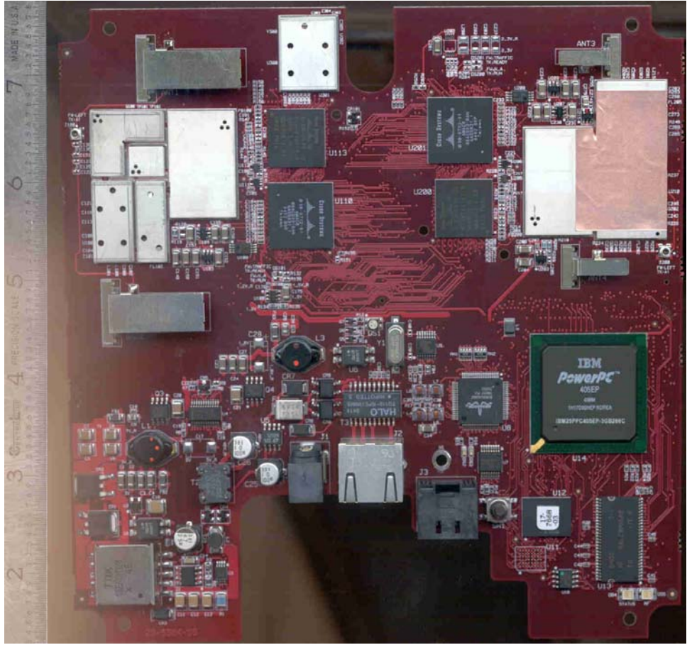
Top with Shields
