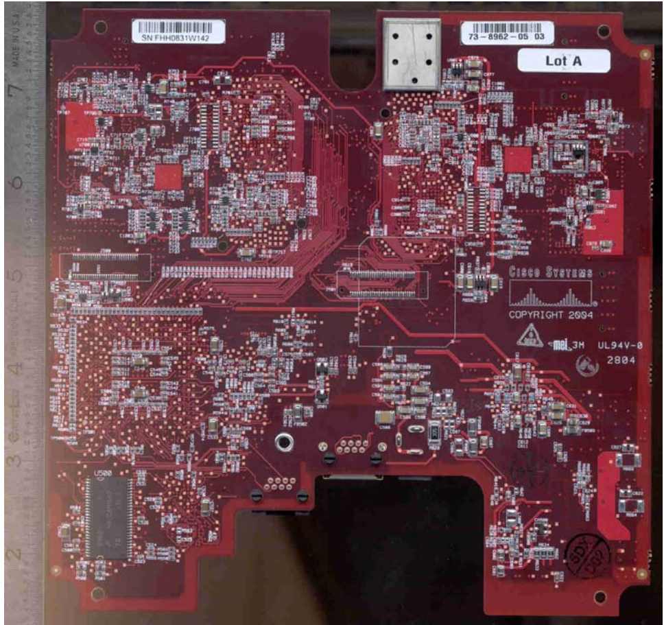
Bottom with Shields
