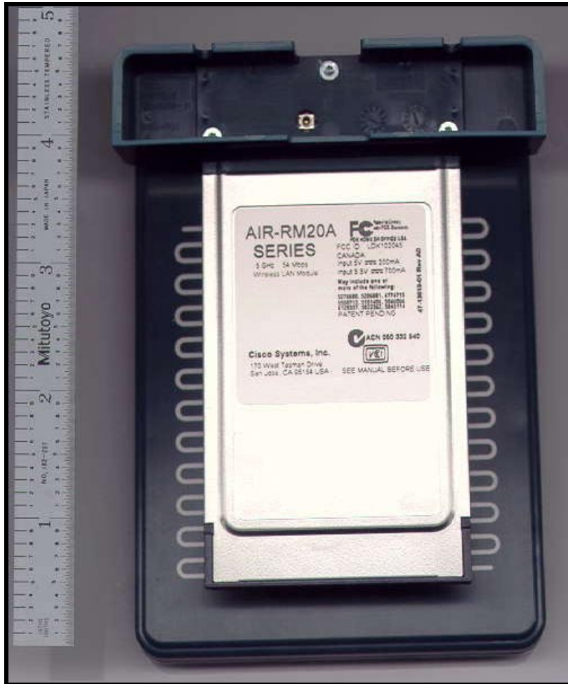
PHOTOGRAPH 8: ASSEMBLY BOTTOM
