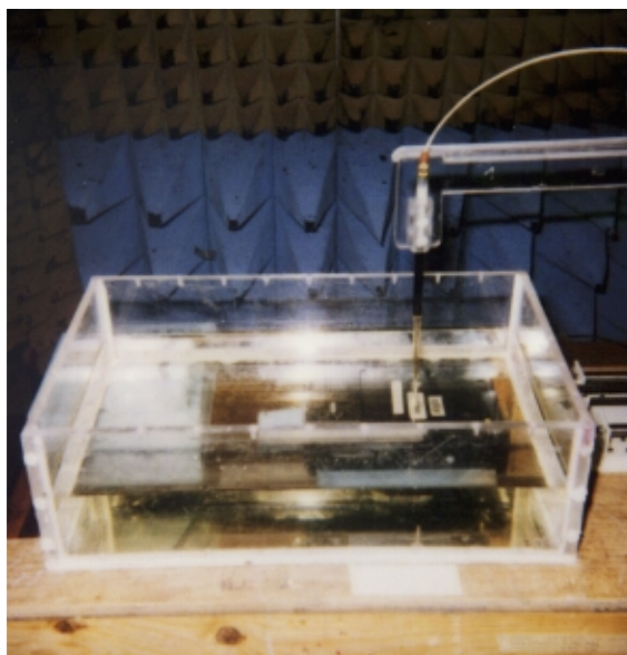
Fig. 2. Photograph of Cisco/Aironet Model LDK102038 Wireless PC mounted with its bottom pressed against the bottom of the planar tissue-simulant phantom.
