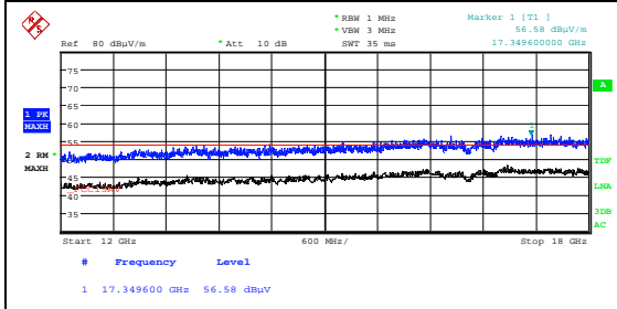
Radiated Emissions 12-18 GHz, Ch93, 802.11ax HT20 Ant1, HP
