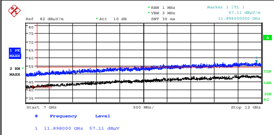
Radiated Emissions 7-12 GHz, Ch93, 802.11ax HT20 Ant0, HP
