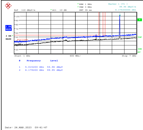
Radiated Emissions 1-7 GHz, Ch45, 802.11ax HT20 MIMO, HP
