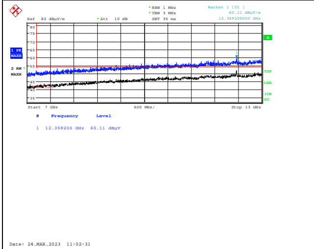
Radiated Emissions 7-13 GHz, Ch45, 802.11ax HT20 Ant1, HP
