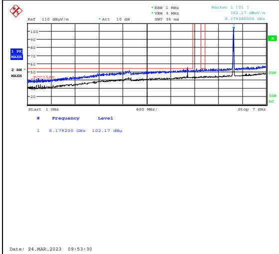
Radiated Emissions 1-7 GHz, Ch45, 802.11ax HT20 Ant1, HP
