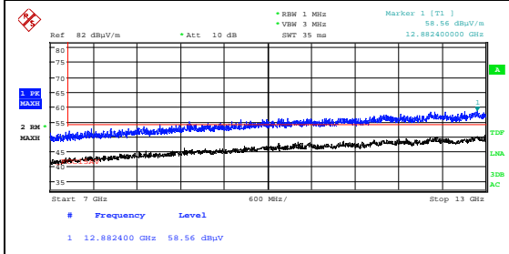
Radiated Emissions 7-13 GHz, Ch43, 802.11ax HT40 Ant0, HP
