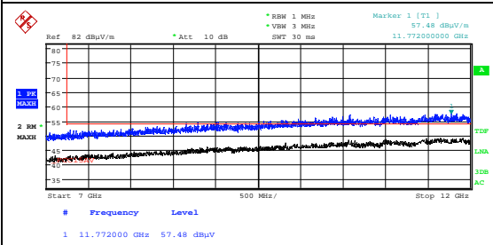
Radiated Emissions 7-12 GHz, Ch93, 802.11ax HT20 Ant1, HP
