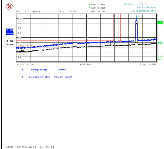
Radiated Emissions 1-7 GHz, Ch39, 802.11ax HT80 Ant1, HP
