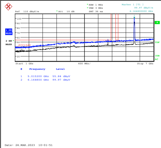
Radiated Emissions 1-7 GHz, Ch43, 802.11ax HT40 MIMO, HP
