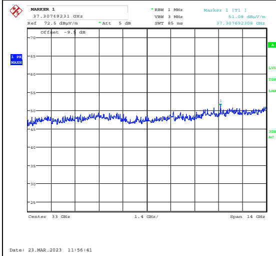
Radiated Emissions 26-40 GHz, Ch45, 802.11ax HT20 MIMO, HP
