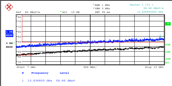
Radiated Emissions 7-13 GHz, Ch39, 802.11ax HT80 Ant1, HP
