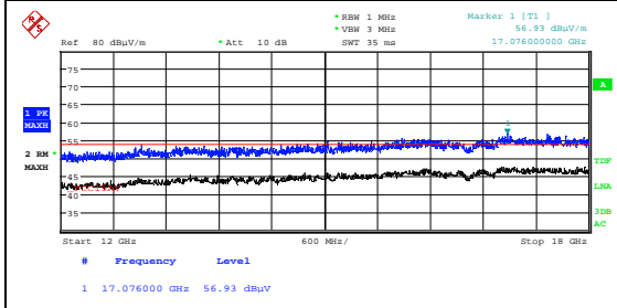
Radiated Emissions 12-18 GHz, Ch93, 802.11ax HT20 Ant0, HP
