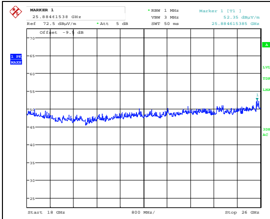
Radiated Emissions 18-26 GHz, Ch45, 802.11ax HT20 Ant0, HP
