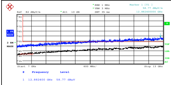
Radiated Emissions 7-13 GHz, Ch43, 802.11ax HT40 Ant1, HP
