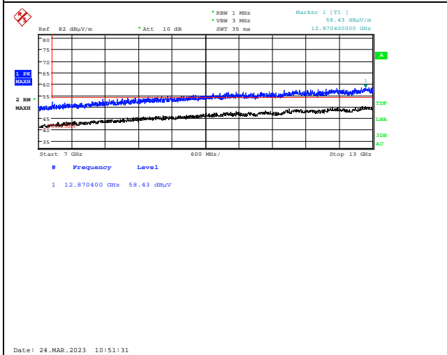
Radiated Emissions 7-13 GHz, Ch45, 802.11ax HT20 MIMO, HP
