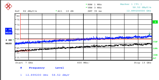
Radiated Emissions 7-13 GHz, Ch39, 802.11ax HT80 Ant0, HP
