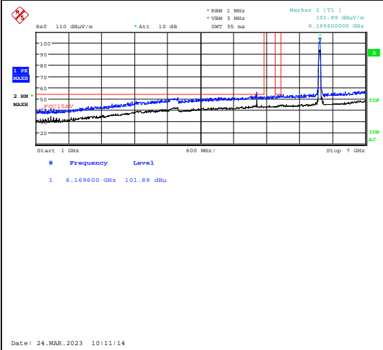
Radiated Emissions 1-7 GHz, Ch43, 802.11ax HT40 Ant1, HP
