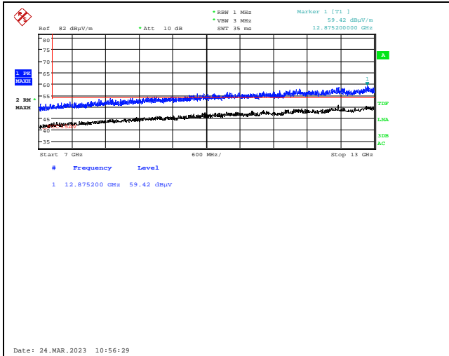
Radiated Emissions 7-13 GHz, Ch45, 802.11ax HT20 Ant0, HP
