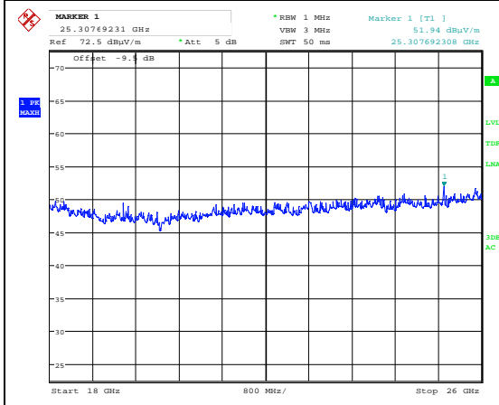
Radiated Emissions 18-26 GHz, Ch45, 802.11ax HT20 Ant1, HP
