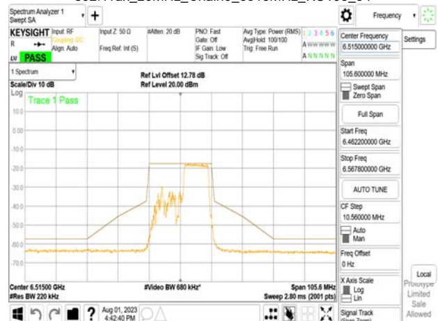
802.11ax_20MHz_Chain0_6515MHz_RU106_54
