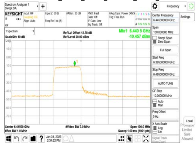
802.11ax_40MHz_Chain1_6445MHz_RU242_61
