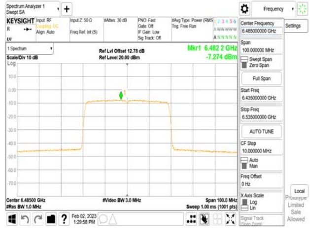
802.11ax_40MHz_Chain0_6485MHz_RU242_62
