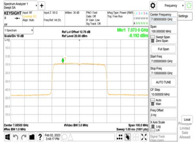
802.11ax_40MHz_Chain0_7085MHz_RU242_62
