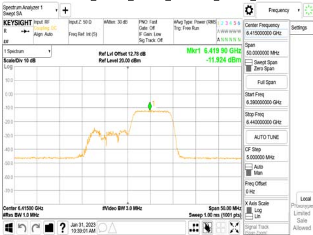
802.11ax_20MHz_Chain0_6415MHz_RU106_54
