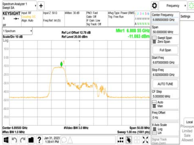
802.11ax_20MHz_Chain0_6895MHz_RU106_53
