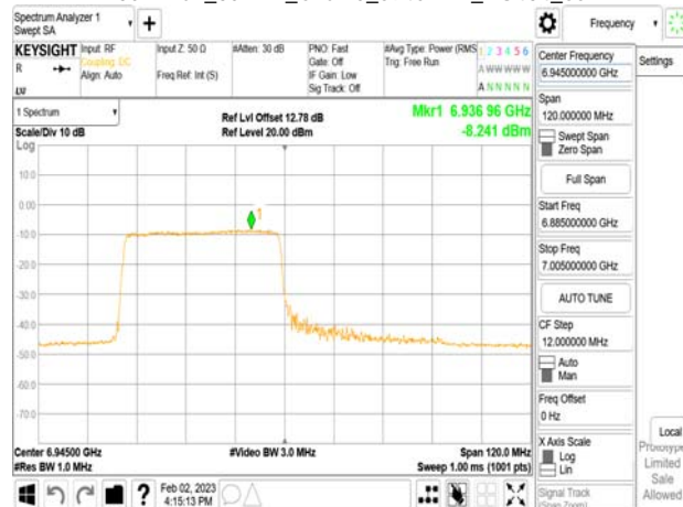
802.11ax_80MHz_Chain0_7025MHz
