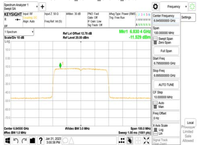
802.11ax_40MHz_Chain0_6845MHz_RU242_62
