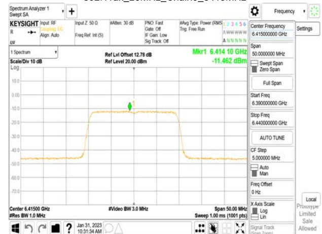
802.11ax_20MHz_Chain0_6415MHz
