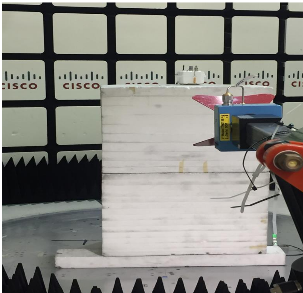
Radiated Emissions above 1GHz
