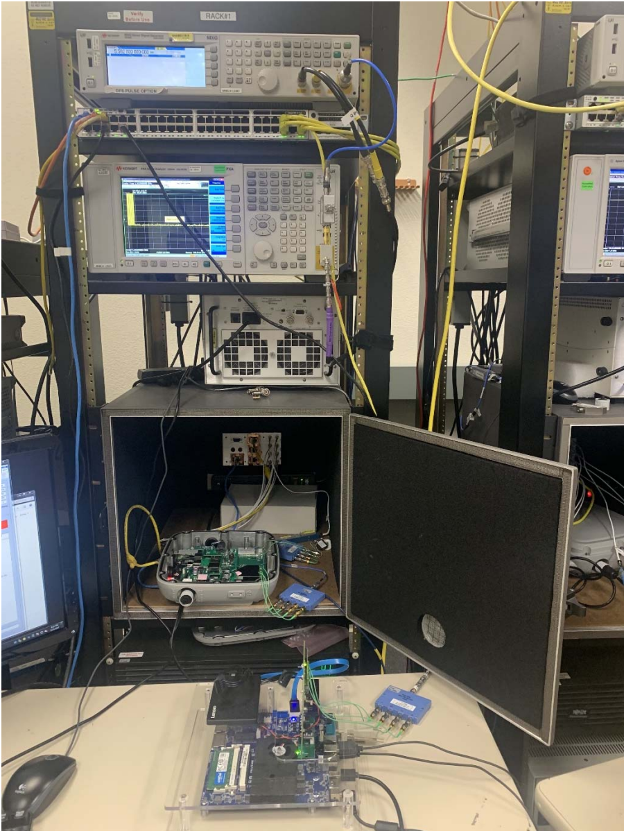
Title: Radio Conducted DFS Test Setup
