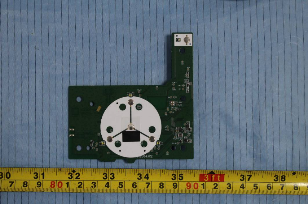
EUT –Main Board Bottom View 1
