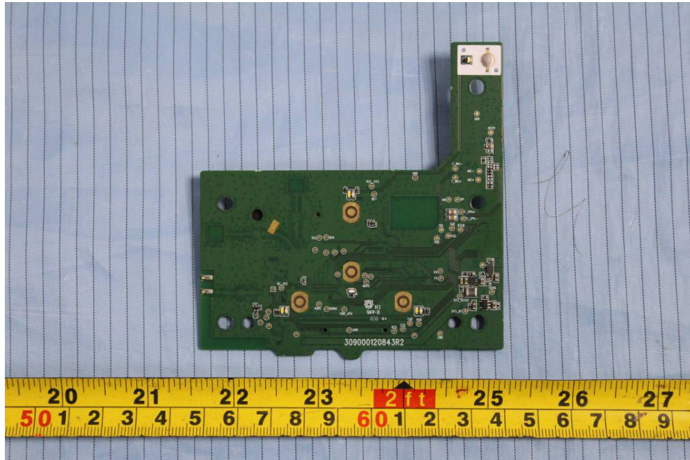
EUT –Main Board Bottom View 2
