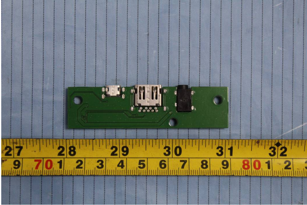
EUT – Ports Board Bottom View
