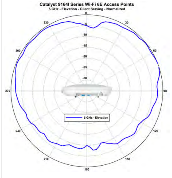
Figure 6: CW9164I - Client-Serving Normalized Radiation Pattern (5-GHz Elevation)
