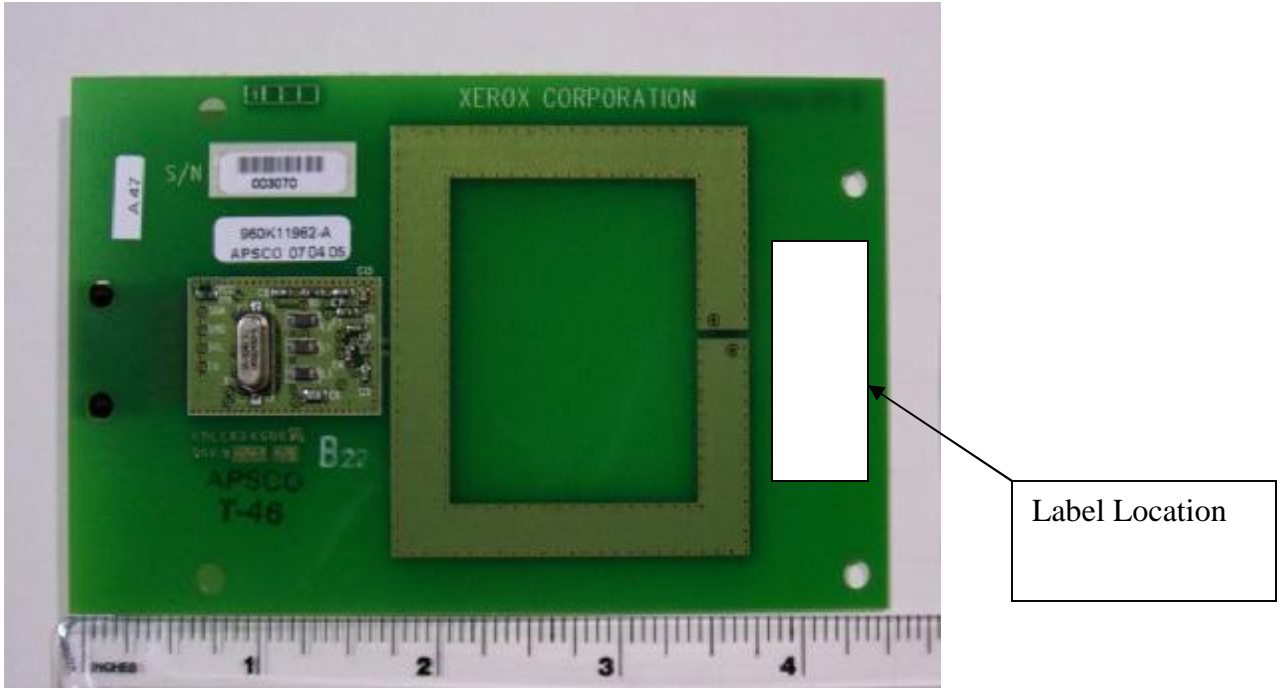
Label Location
