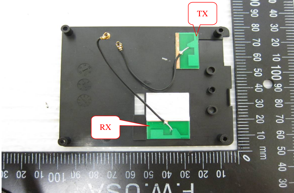
Internal View of EUT – 4 (WiFi antenna)
