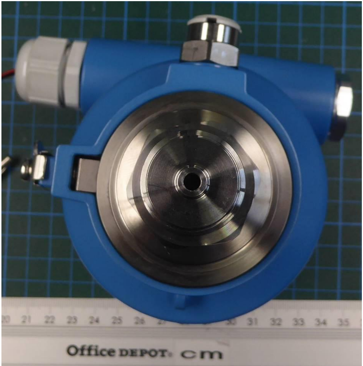
EUT VE113_A_03 in representative housing – back view
