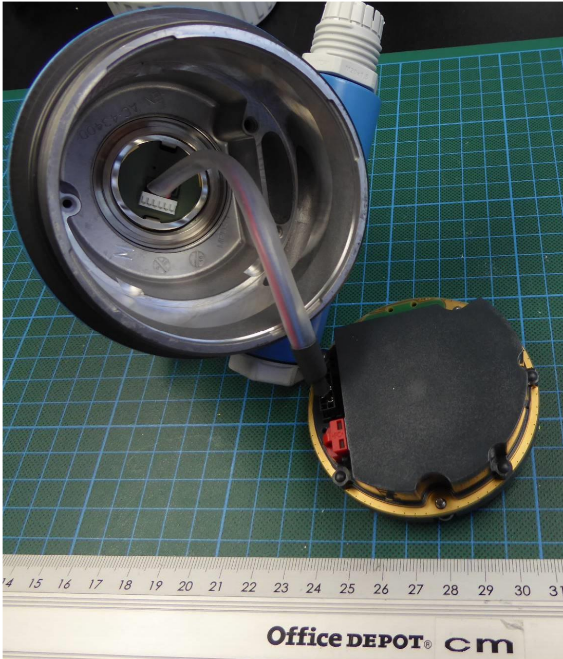
Housing open 4
