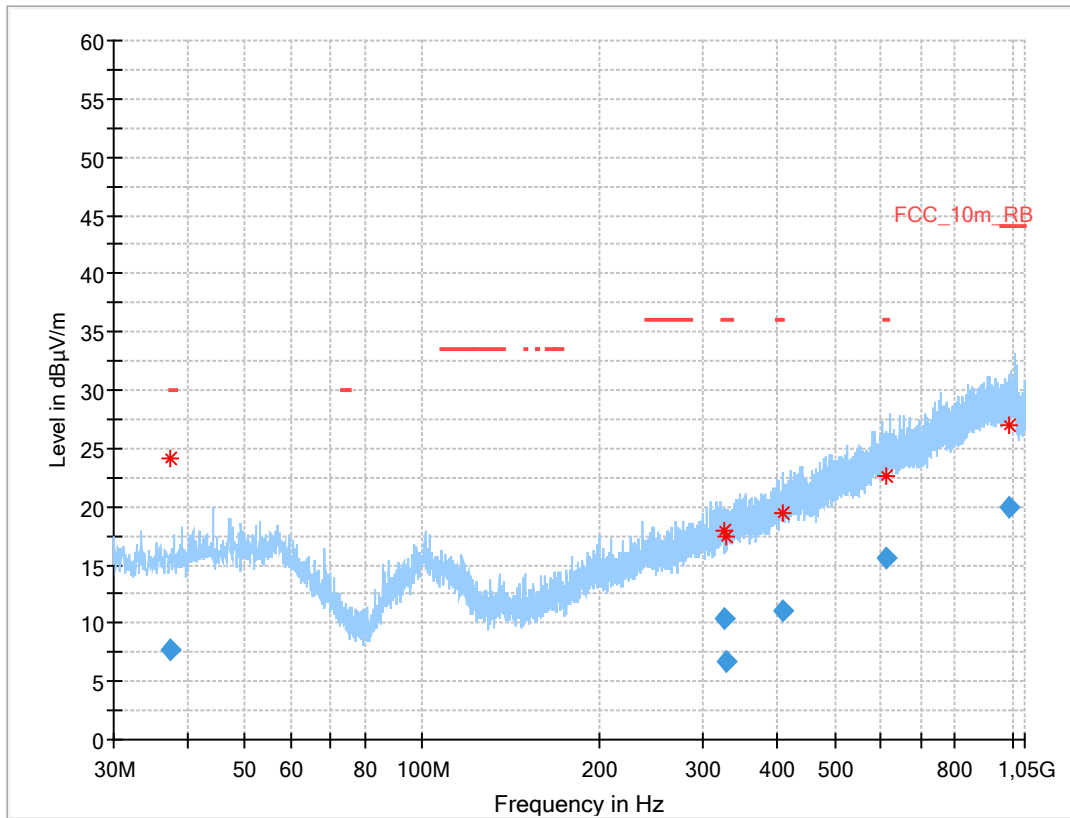
Plot 2: 30 MHz to 1 GHz, vertical & horizontal polarization, DSSS mode
