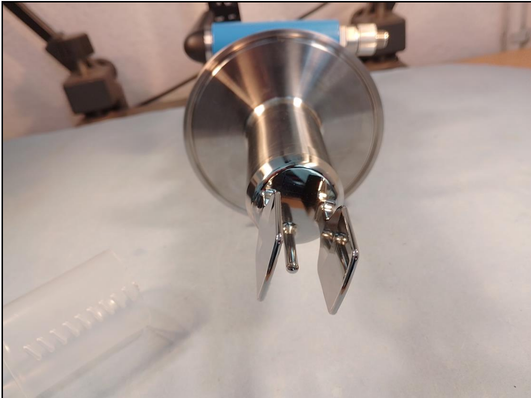
Photo 8: EUT
