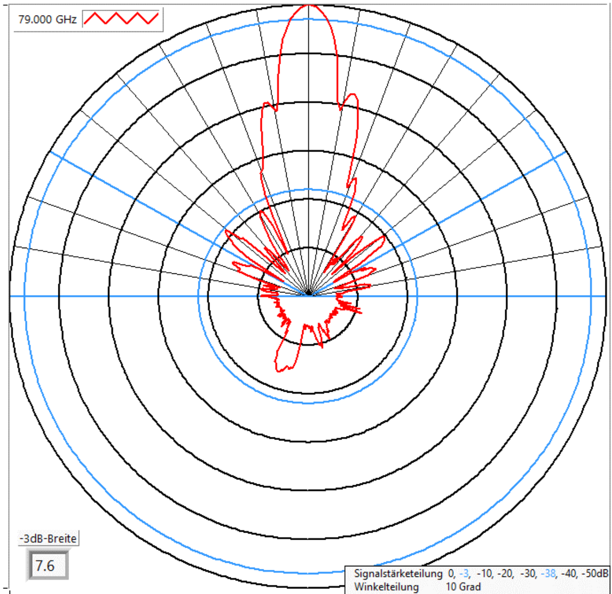
Antenna diagram as provided by the applicant in the H-plane
