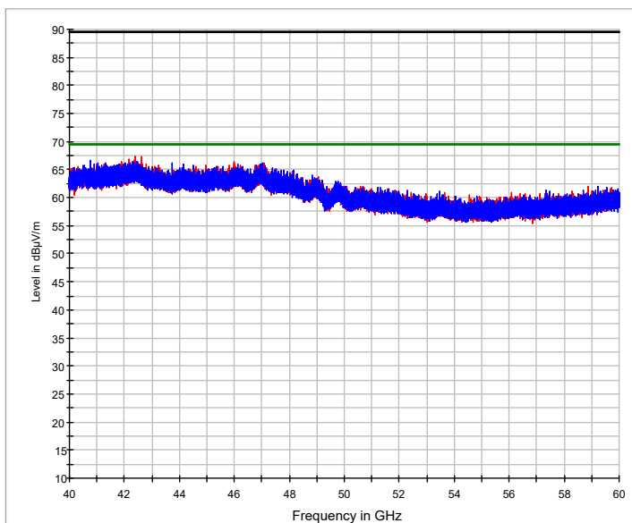
— Preview Result 2H-AVG — Preview Result 2V-AVG — FCC 15.209 (0.5m) PK — FCC 15.209 (0.5m) AV * Final_Result PK+ ◊ Final_Result AVG
