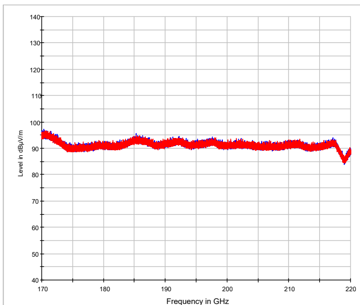
Preview Result 1V-PK+ Preview Result 1H-PK+
