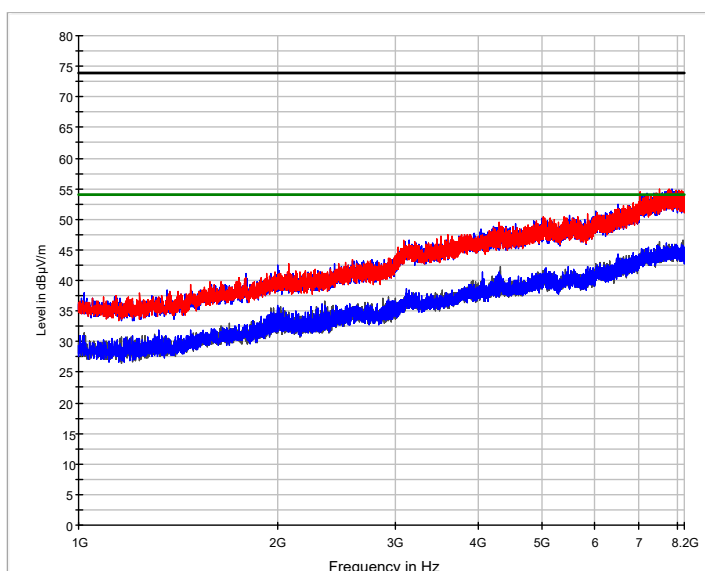
— Preview Result 2V-AVG — Preview Result 1V-PK+ — Preview Result 2H-AVG * Final_Result PK+ ◊ Final_Result AVG — FCC 15.209 PK — FCC 15.209 AV
