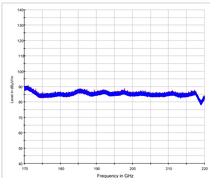
Preview Result 1H-AVG Preview Result 1V-AVG
