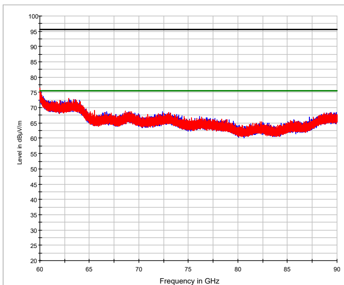
— Preview Result 1V-AVG — Preview Result 1H-AVG — FCC 15.209 (0.25m) PK — FCC 15.209 (0.25m) AV * Final_Result AVG
