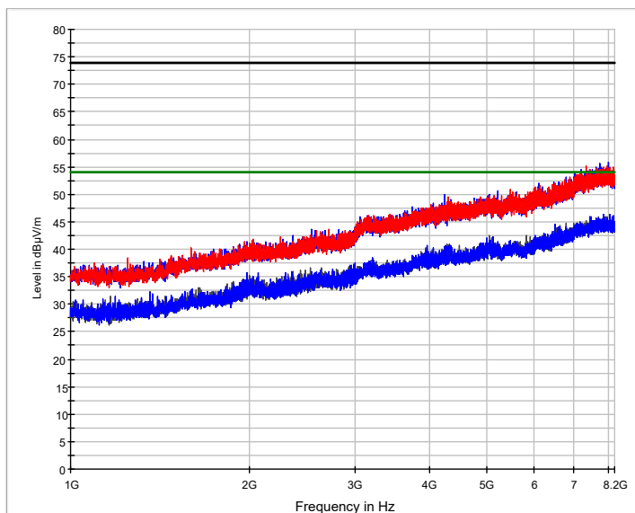
— Preview Result 2V-AVG — Preview Result 1V-PK+ — Preview Result 2H-AVG — Preview Result 1H-PK+ — FCC 15.209 PK — FCC 15.209 AV * Final_Result PK+ ◊ Final_Result AVG
