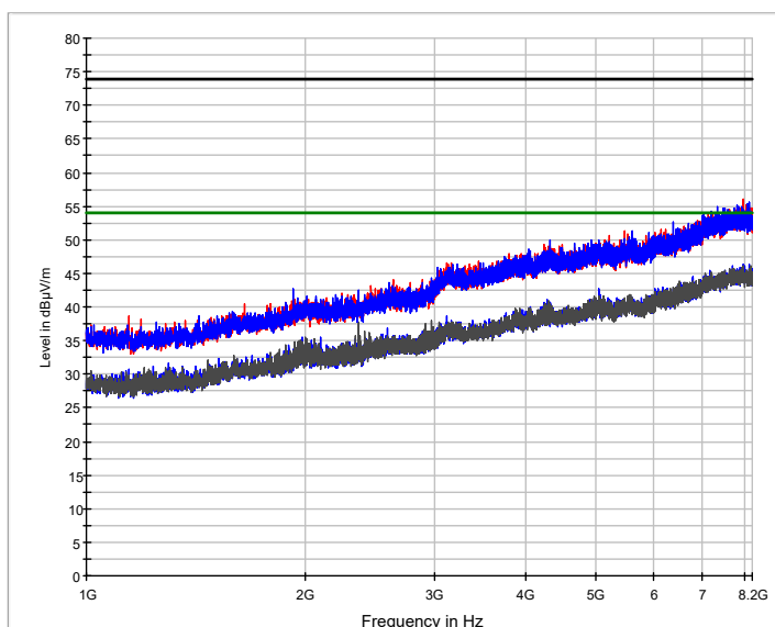
— Preview Result 2H-AVG — Preview Result 1H-PK+ — Preview Result 2V-AVG * Final_Result PK+ ◊ Final_Result AVG — FCC 15.209 AV
