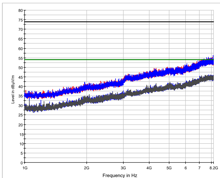
— Preview Result 2H-AVG — Preview Result 1H-PK+ — Preview Result 2V-AVG — Preview Result 1V-PK+ — FCC 15.209 PK — FCC 15.209 AV * Final_Result PK+ ◊ Final_Result AVG
