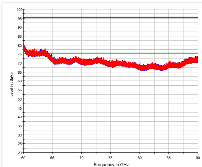
— Preview Result 1V-PK+ — Preview Result 1H-PK+ — FCC 15.209 (0.25m) PK — FCC 15.209 (0.25m) AV
