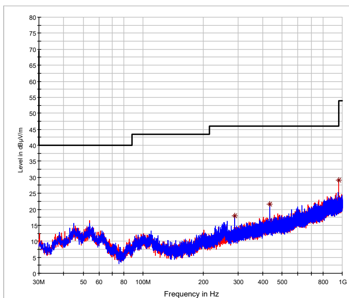
— Preview Result 1H-PK+ — Preview Result 1V-PK+ — FCC 15.209 * Final_Result PK
