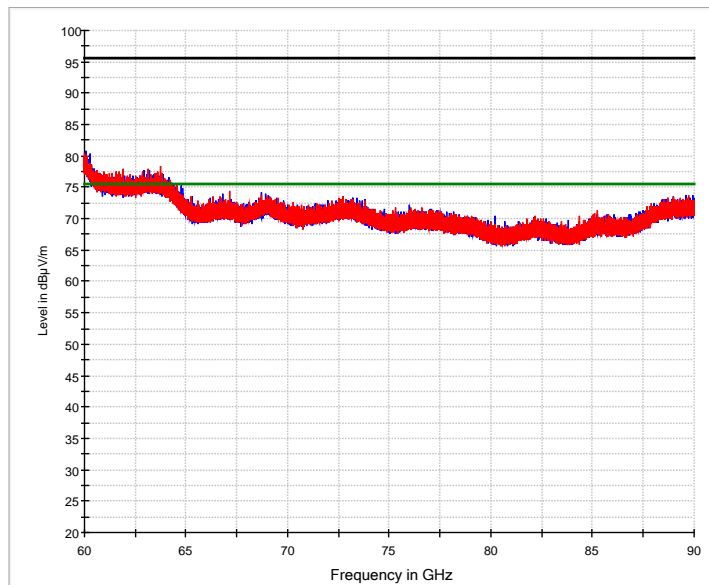
— Preview Result 1V-PK+ FCC 15.209 (0.25m) PK — Preview Result 1H-PK+ FCC 15.209 (0.25m) AV — FCC 15.209 (0.25m) AV — FCC 15.209 (0.25m) PK
