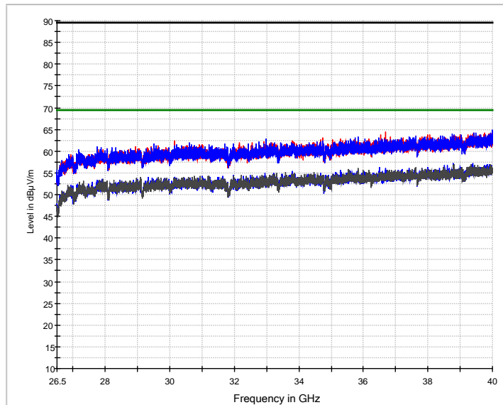
— Preview Result 2H-AVG — Preview Result 1H-PK+ — Preview Result 2V-AVG — Preview Result 1V-PK+ — FCC 15.209 (0.5m) PK — FCC 15.209 (0.5m) AV * Final_Result PK+ ◇ Final_Result AVG
