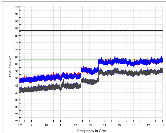
— Preview Result 2H-AVG — Preview Result 1H-PK+ — Preview Result 2V-AVG — Preview Result 1V-PK+ — FCC 15.209 (1m) PK — FCC 15.209 (1m) AV * Final_Result PK+ ◇ Final_Result AVG
