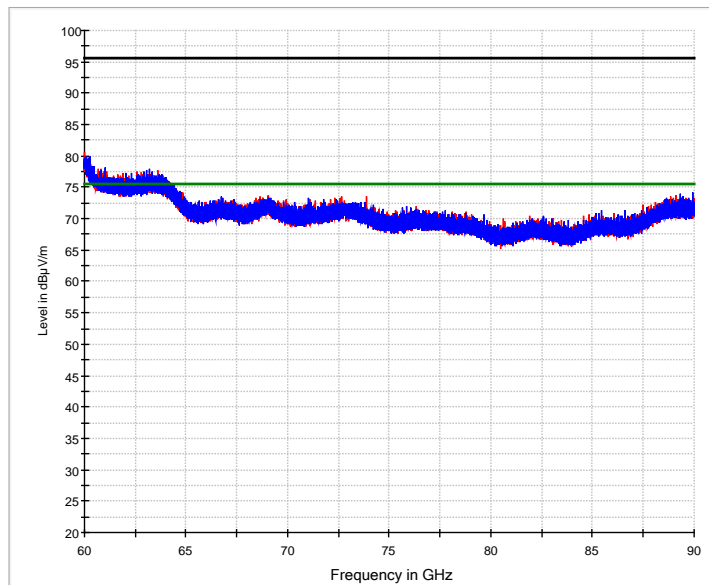
— Preview Result 1H-PK+ FCC 15.209 (0.25m) PK — Preview Result 1V-PK+ FCC 15.209 (0.25m) AV — —
