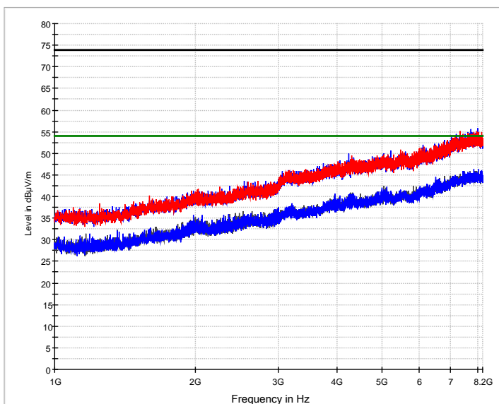
— Preview Result 2V-AVG — Preview Result 1V-PK+ — Preview Result 2H-AVG * Final_Result PK+ ◊ Final_Result AVG — FCC 15.209 AV
