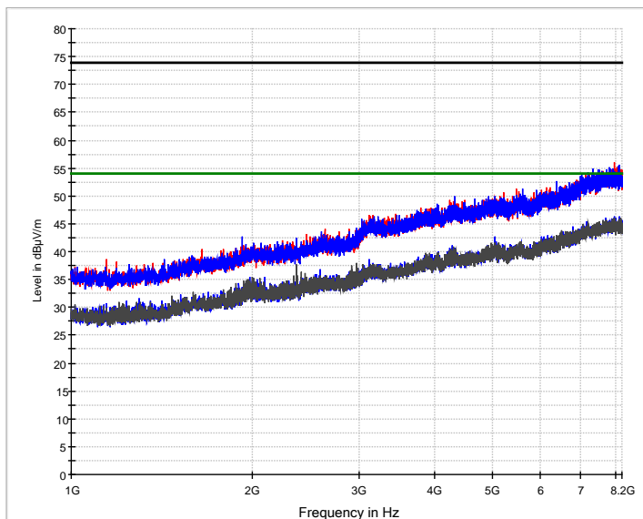
— Preview Result 2H-AVG — Preview Result 1H-PK+ — Preview Result 2V-AVG * Final_Result PK ♦ Final_Result AVG — FCC 15.209 PK — FCC 15.209 AV
