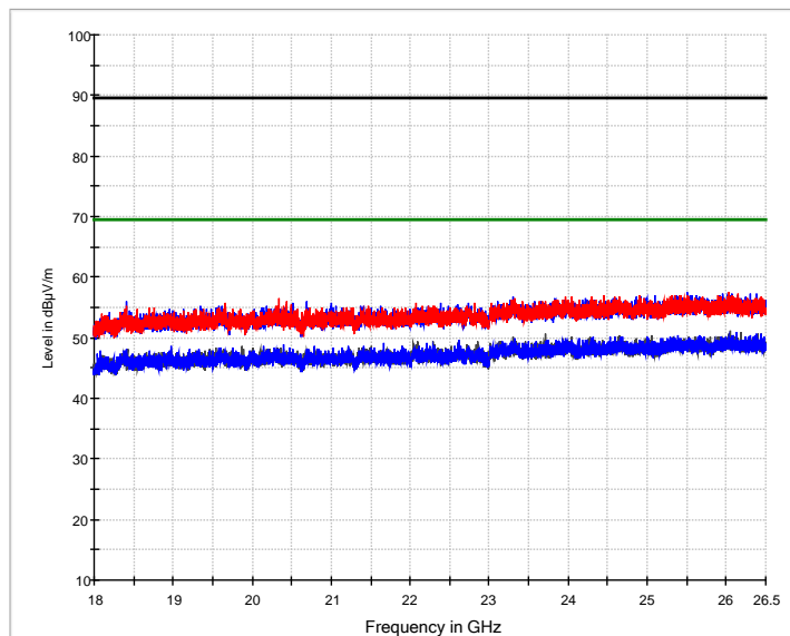
— Preview Result 2V-AVG — Preview Result 1V-PK+ — Preview Result 2H-AVG — Preview Result 1H-PK+ — FCC 15.209 (0.5m) PK — FCC 15.209 (0.5m) AV * Final_Result PK+ ◇ Final_Result AVG
