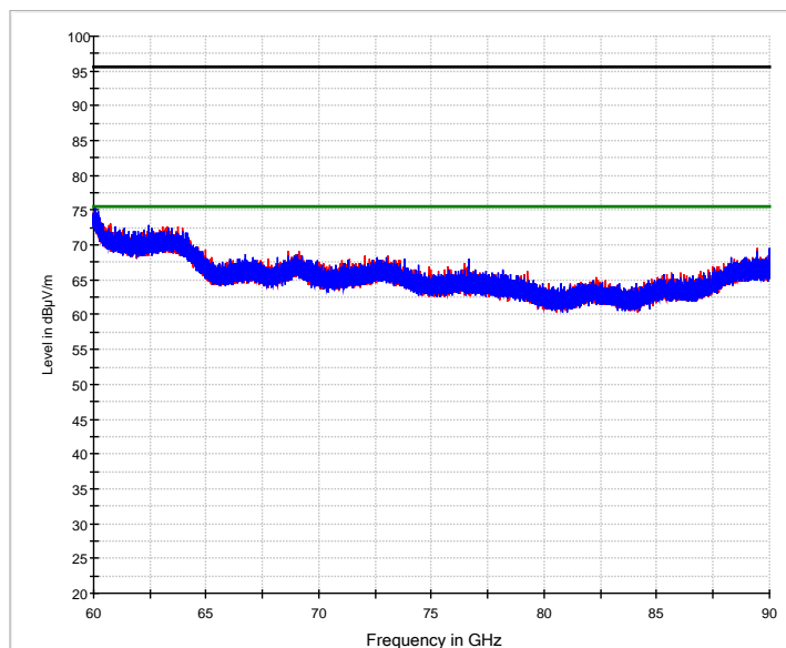
— Preview Result 1H-AVG — Preview Result 1V-AVG — FCC 15.209 (0.25m) PK — FCC 15.209 (0.25m) AV * Average-AVG
