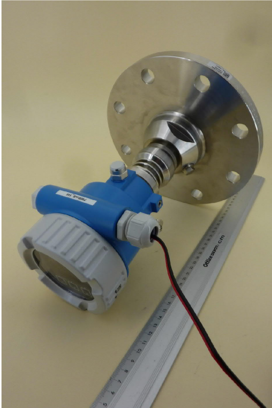
EUT 8, 3-D-view 1
