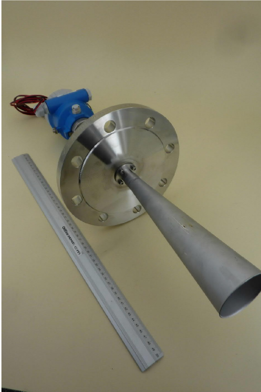
EUT 6, 3-D-view 2
