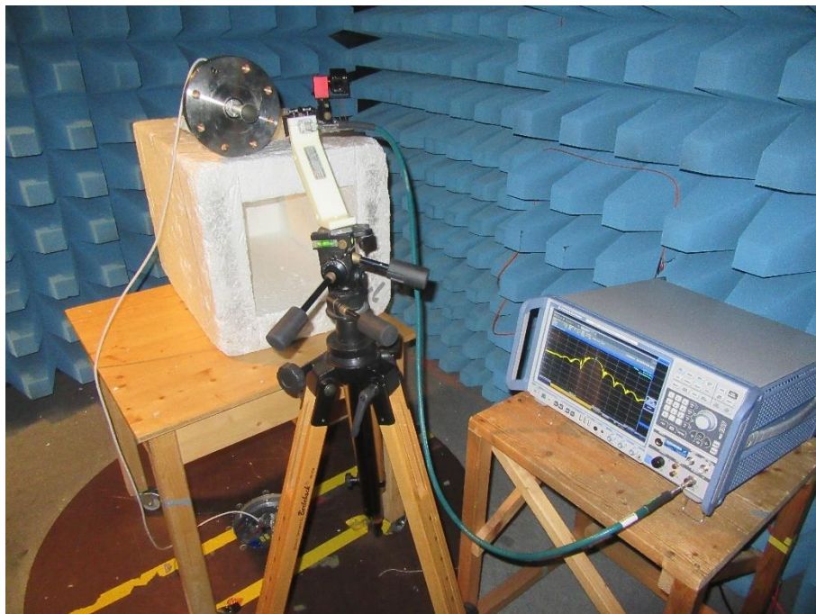
Figure 13 - Test setup for 24.05-29.00 GHz band specific tests
