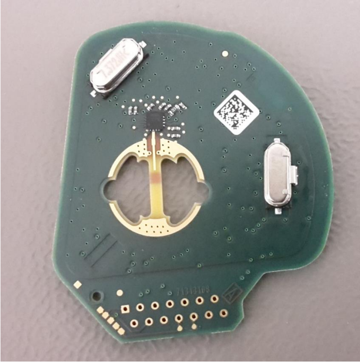
RF board bottom:
