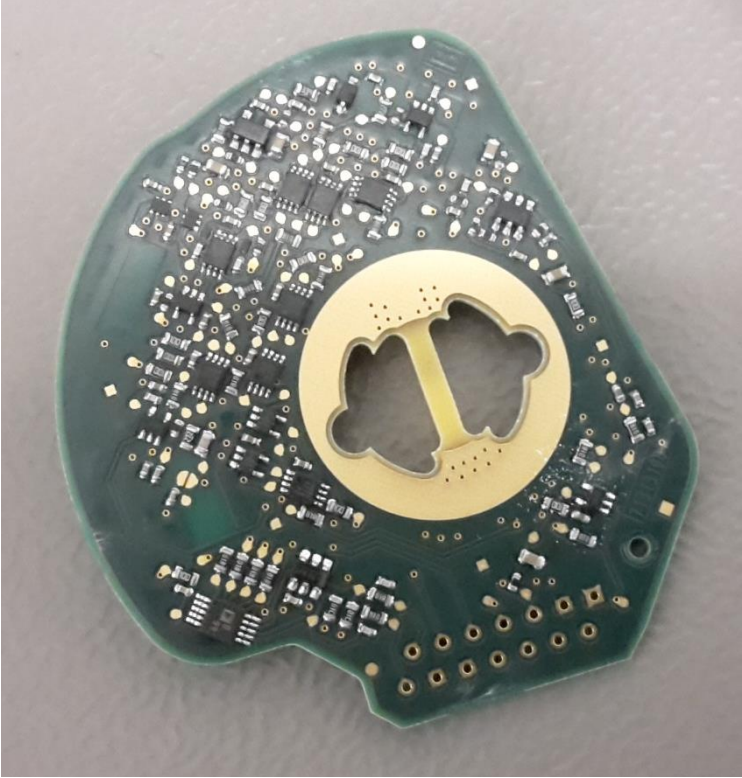
RF board top:
