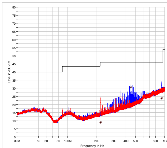
◇ Preview Result 1V-PK+ Final_Result AVG — FCC 15.209_3m — Preview Result 1H-PK+ * Final_Result QPK
