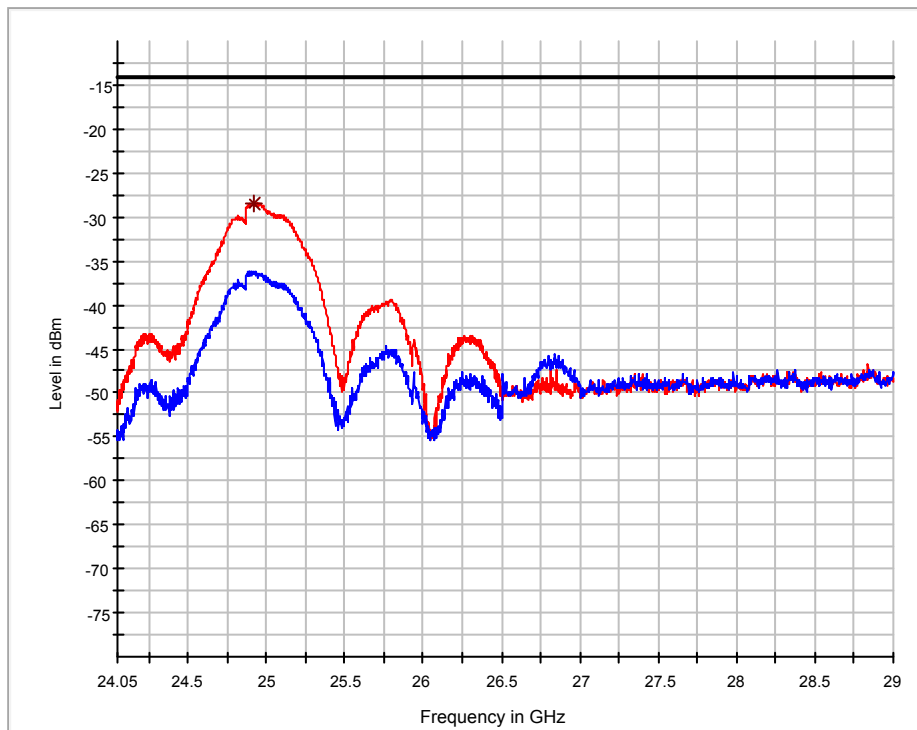
— Preview Result 1H-RMS — Preview Result 1V-RMS EN 302 729 in beam 25GHz * Final_Result RMS
