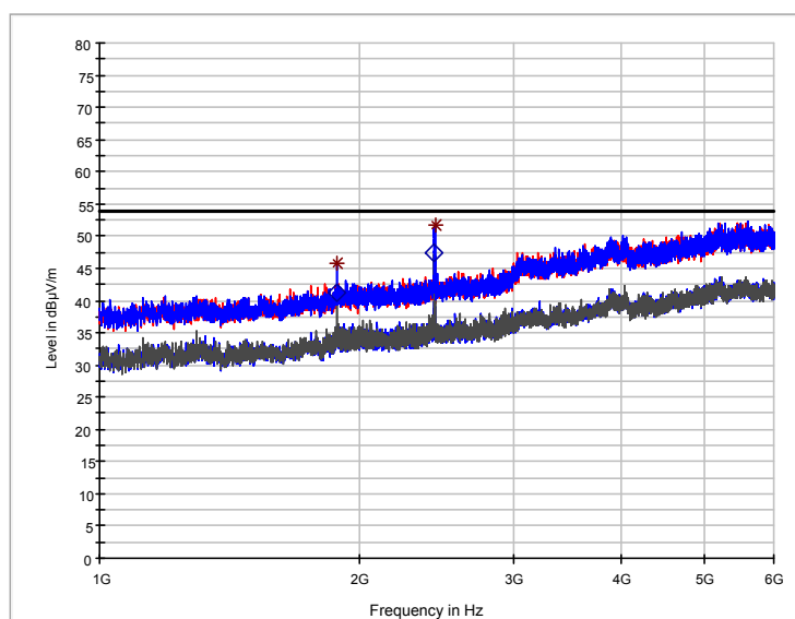
◇ Preview Result 2H-AVG — Preview Result 1H-PK+ — Preview Result 2V-AVG — Preview Result 1V-PK+ — FCC 15.209 * Final_Result PK+
