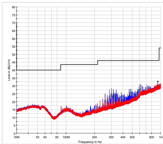
◇ Preview Result 1V-PK+ Final Result AVG — FCC 15.209_3m * Final Result QPK — Preview Result 1H-PK+
