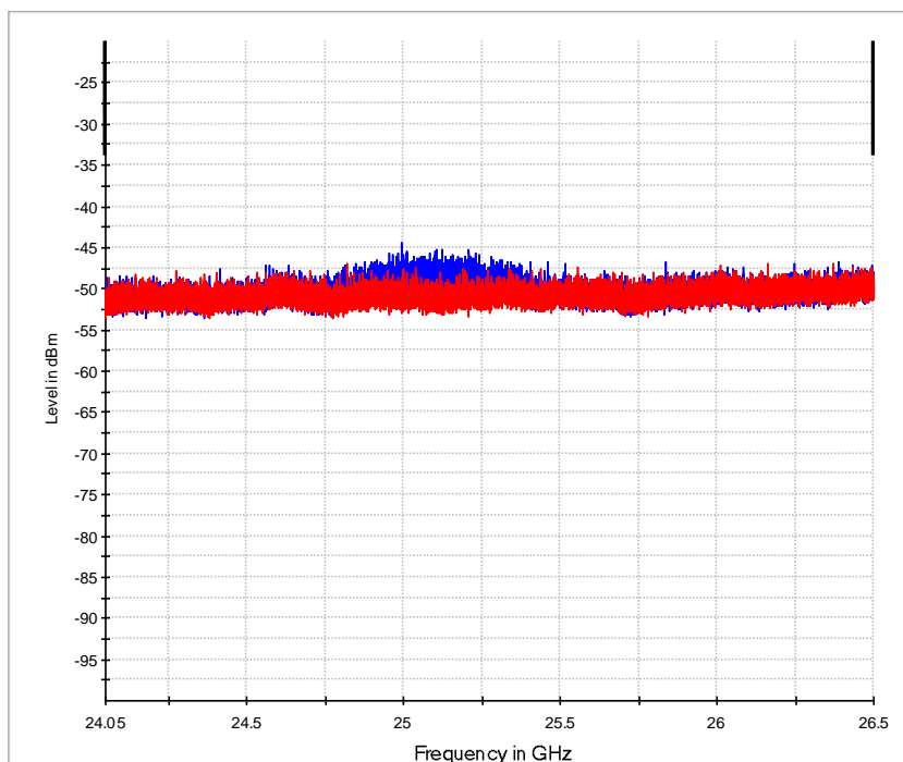
— Preview Result 1V-RMS — Preview Result 1H-RMS EN 302 729 in beam 25GHz
