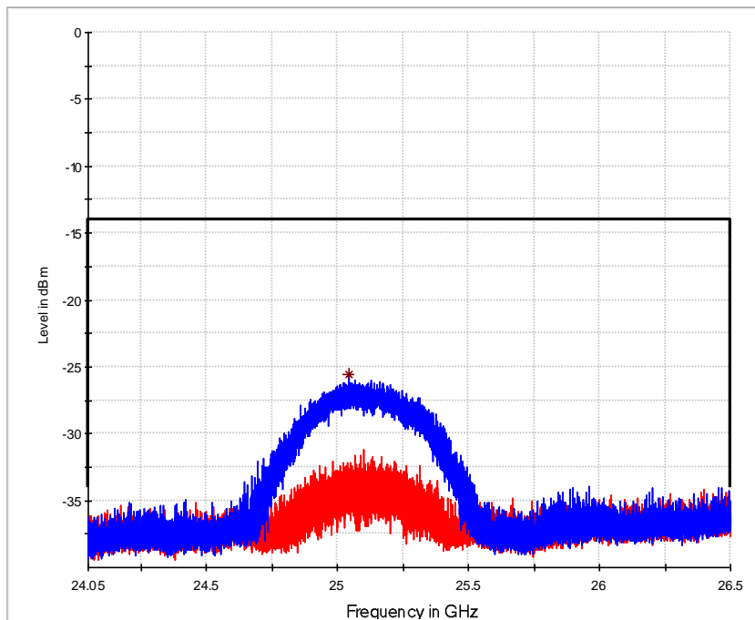
— Preview Result 1H-PK+ — Preview Result 1V-PK+ EN 302 729 in beam 25GHz * Final_Result PK+
