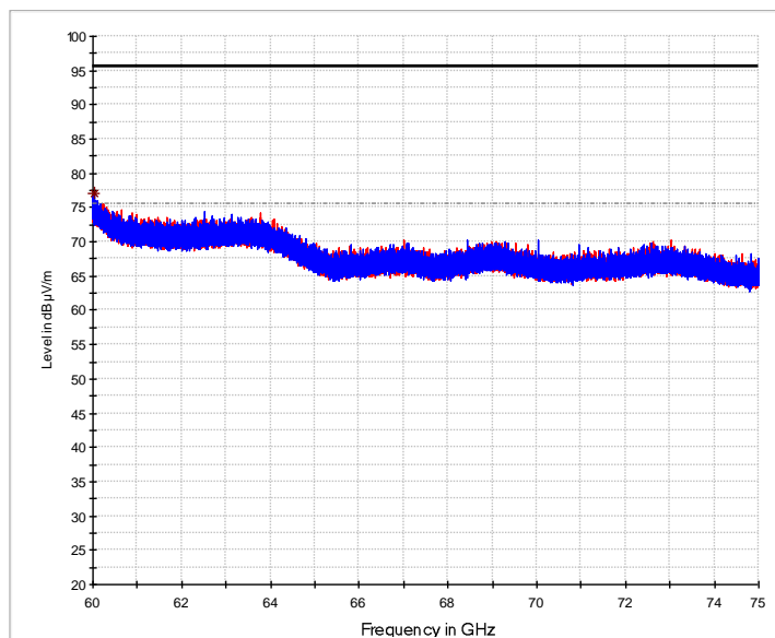
— Preview Result 1H-AVG — Preview Result 1V-AVG — FCC 15.209 (0.25m) PK * * * Final_Result AVG
