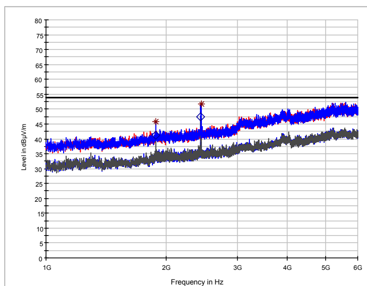
◇ Preview Result 2H-AVG ◇ Preview Result 1V-PK+ ◇ Final_Result AVG — Preview Result 1H-PK+ — FCC 15.209 * Preview Result 2V-AVG * Final_Result PK+
