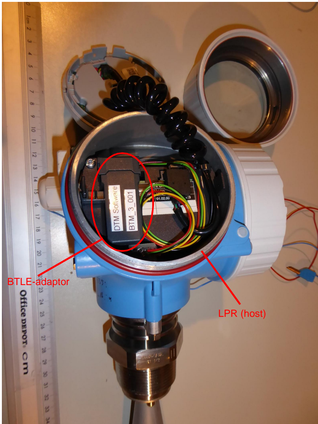
172289_d.JPG: ProToF BTLE-adaptor 2.4 GHz inside FMR51, internal view to mounted BTLE module (display removed)
