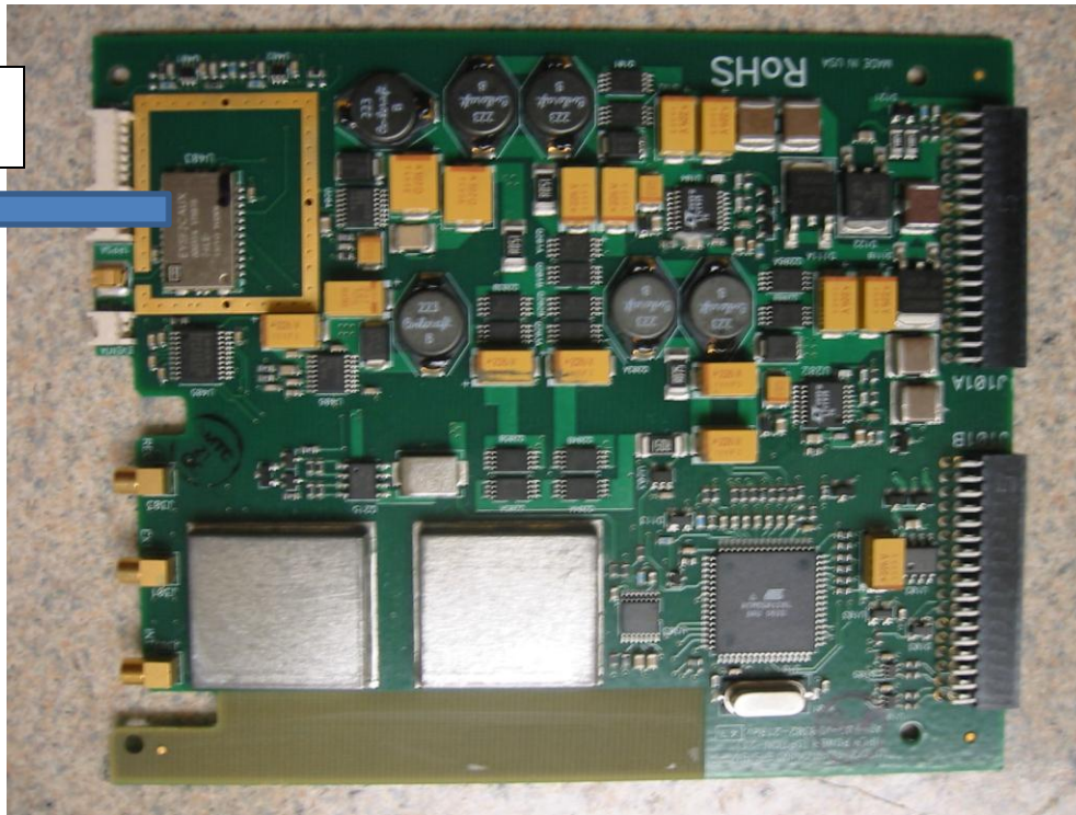
POWER BOARD WITH BLUETOOTH MODULE (with SHIELD)
