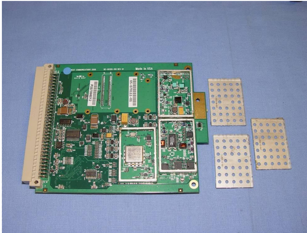
UHF BOARD ASSEMBLY (TOP)
