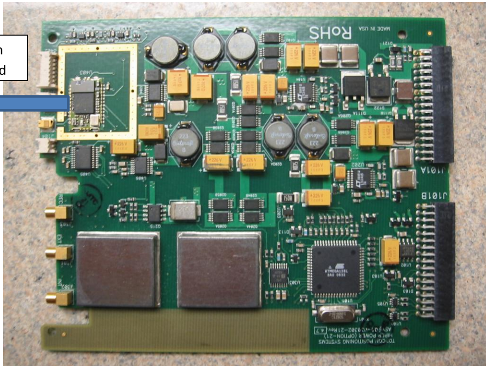
POWER BOARD WITH BLUETOOTH MODULE (WITHOUT SHIELD)
