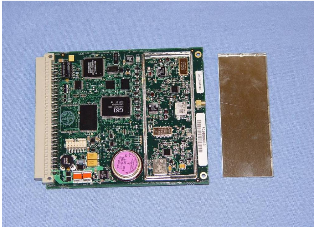
TURBO ASSEMBLY (GPS) -TOP
