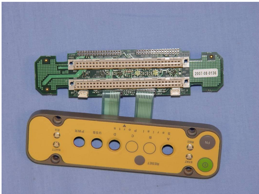
INTERCONNECT ASSEMBLY-REAR
