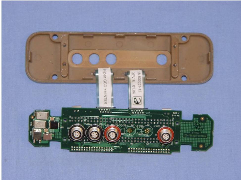
INTERCONNECT ASSEMBLY- FRONT
