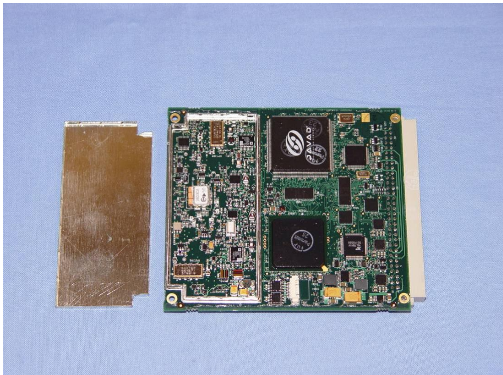
TURBO ASSEMBLY (GPS)- BOTTOM
