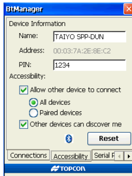
Figure A-2. Check Bluetooth Module Accessibility Settings
