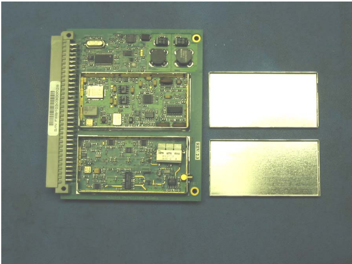
915MHz SS Modem Board
