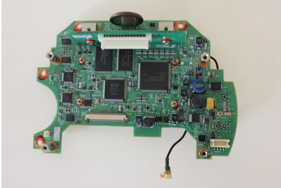
POWER BOARD- TOP
