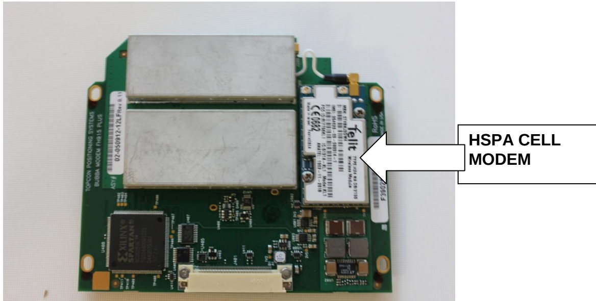
SPREAD SPECTRUM PCBA(FH915+) - TOP - WITH HSPA CELL MODEM
