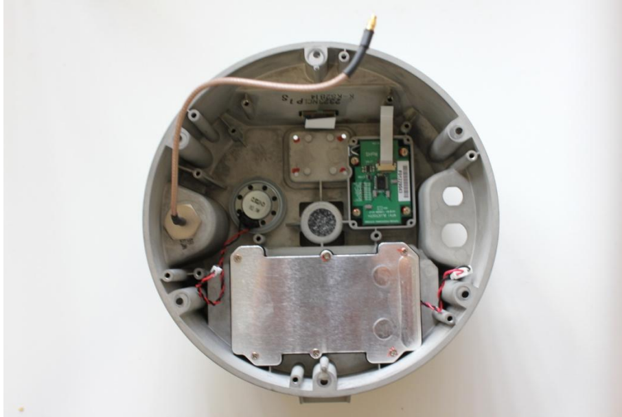
BOTTOM ENCLOSURE WITH BLUETOOTH MODULE
