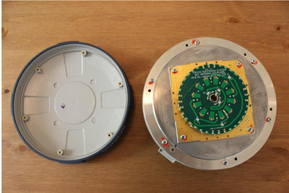
TOP COVER DETACHED
