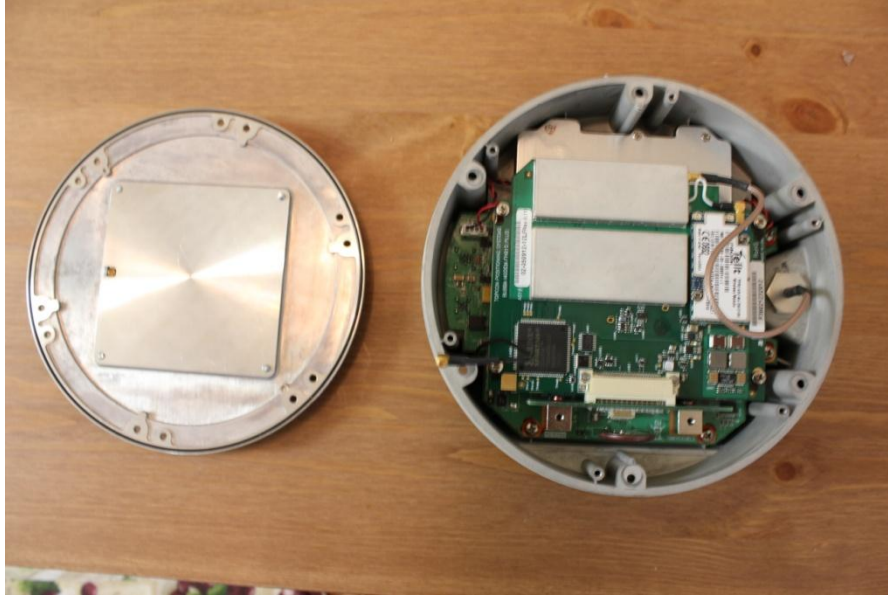
GROUND PLANE DETACHED
