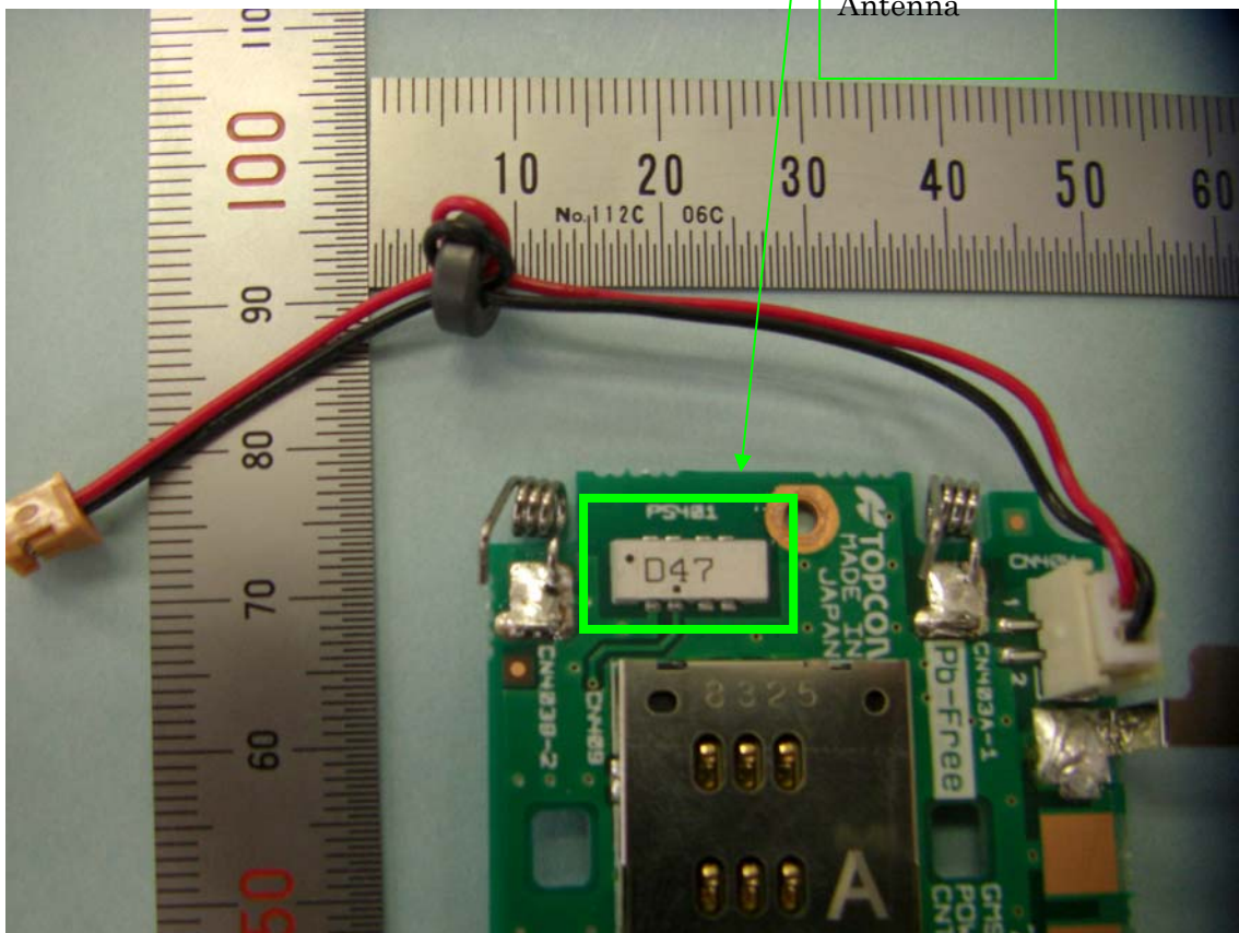
Bluetooth Antenna
