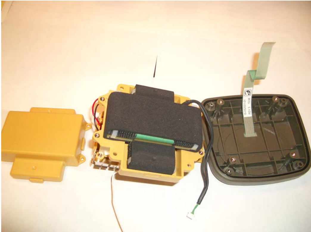
Beacon antenna.
