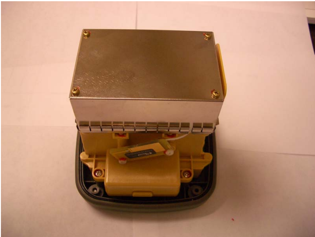
Shielding case and Bluetooth antenna
