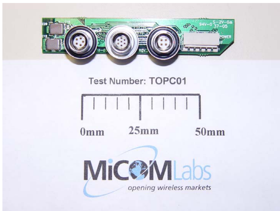
Interconnect Board Top and Bottom
