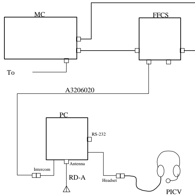
Block Diagram B – Tethered Operation
