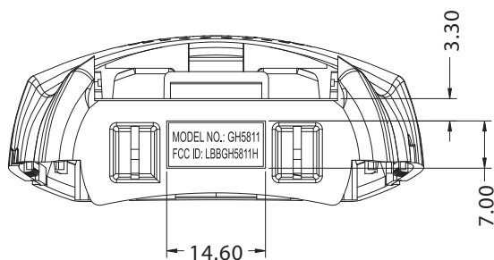
GH5811 HANDSET
