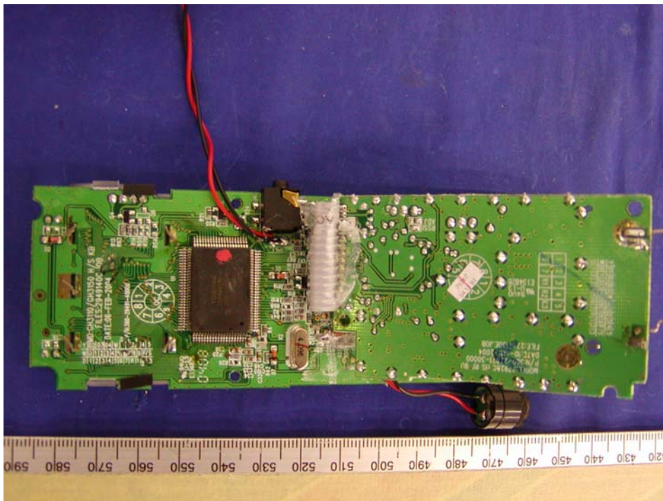
Handset - Component View III (Model: GH3150 & GH3110)
