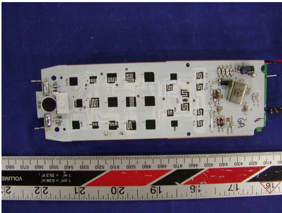
Handset – Main Board Solder View (Model: GH3100)
