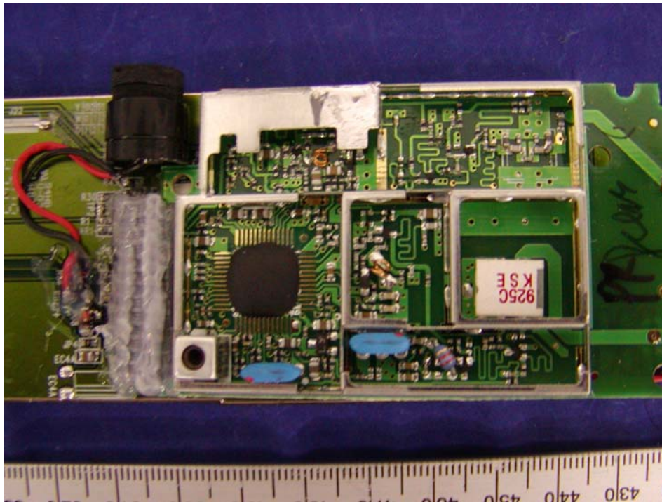
Handset Transceiver - Component View (Model: GH3100)
