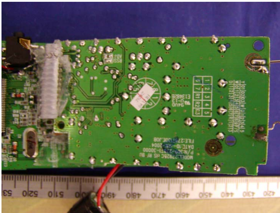
Handset Transceiver - Solder View (Model: GH3150 & GH3110)
