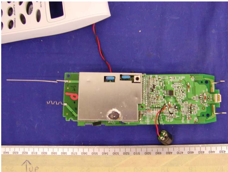
Handset - Component View I (Model: GH3150 & GH3110)
