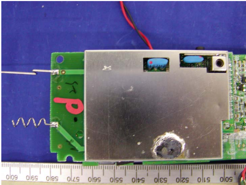
Handset Transceiver - Component View with Shielding (Model: GH3150 & GH3110)
