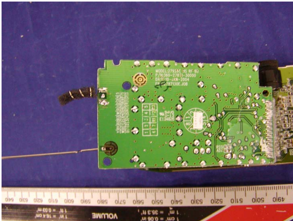
Handset Transceiver – Solder View (Model: GH3100)
