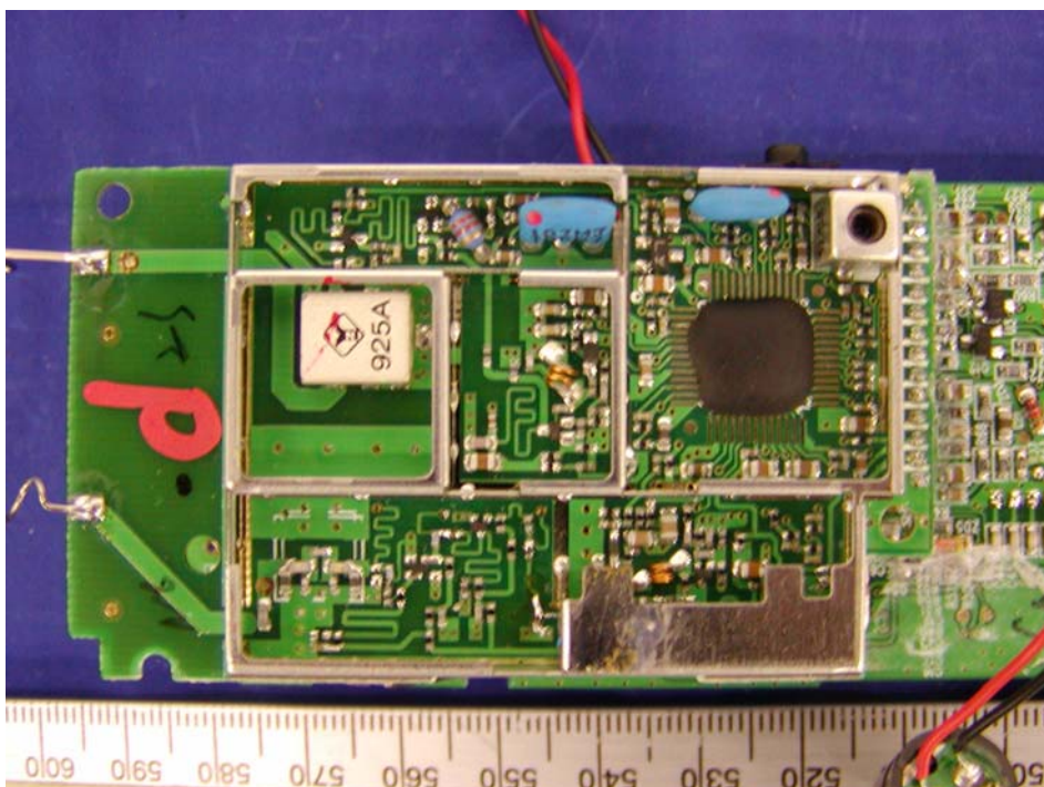
Handset Transceiver - Component View without Shielding (Model: GH3150 & GH3110)
