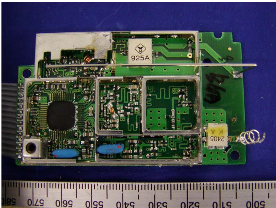
Transceiver – Component View without Shielding (Model: GH3150)
