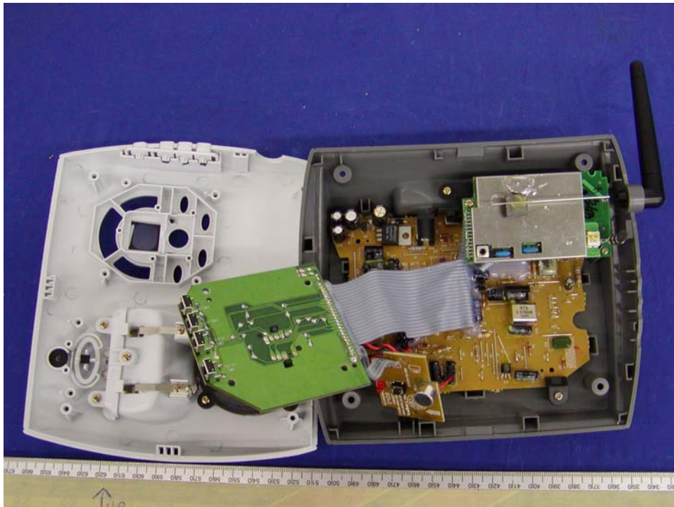
Base – Cover Off View (Model: GH3150)
