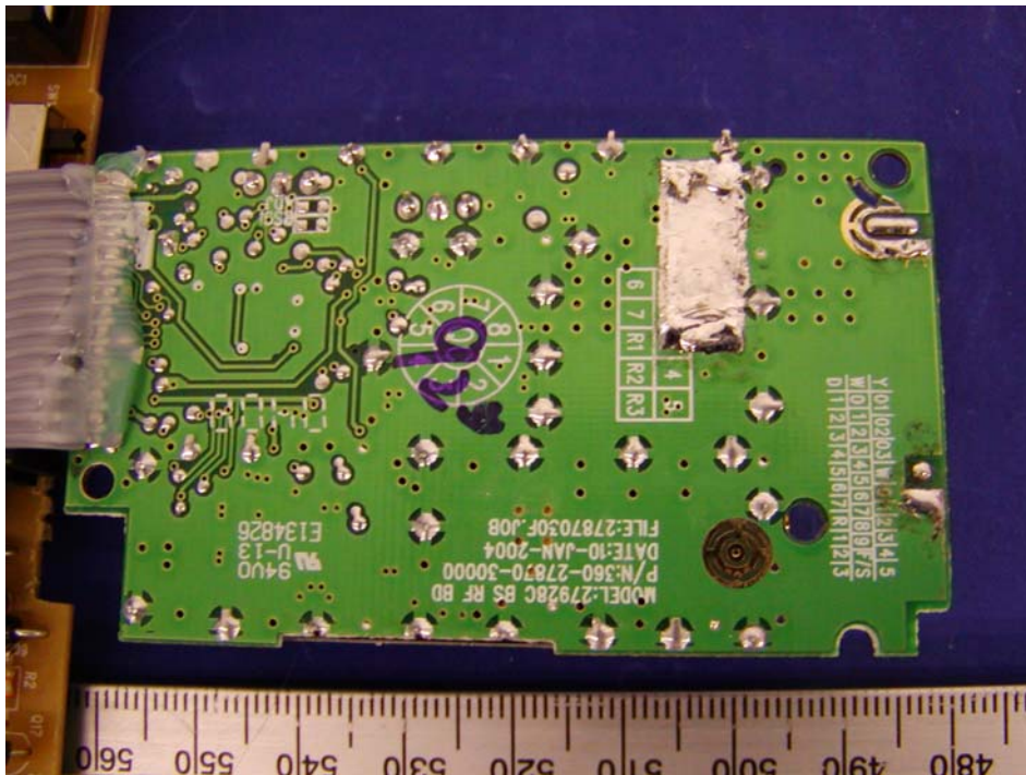
Transceiver – Solder View (Model: GH3150)
