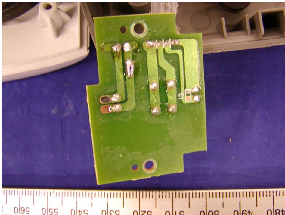
Microphone Board – Solder View (Model: GH3150)
