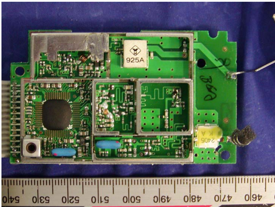
Base Transceiver – Component View (Model: GH3110 & GH3100)
