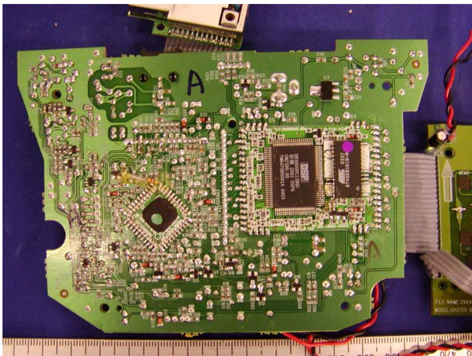
Base – Solder View (Model: GH3150)
