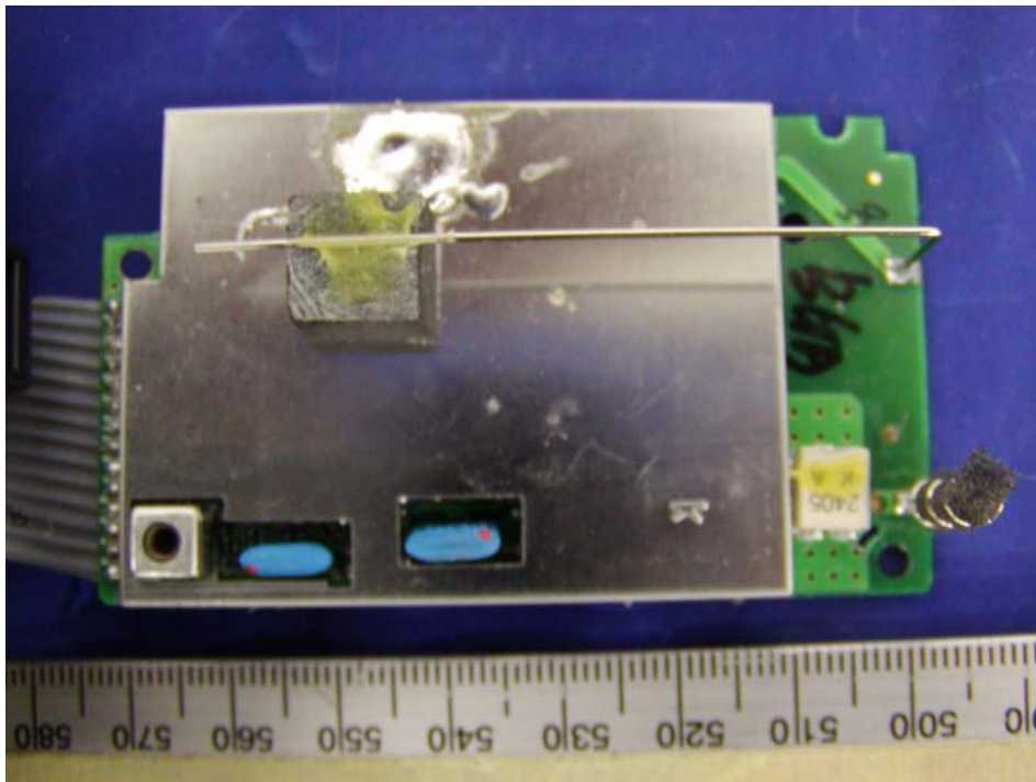
Transceiver – Component View with Shielding (Model: GH3150)
