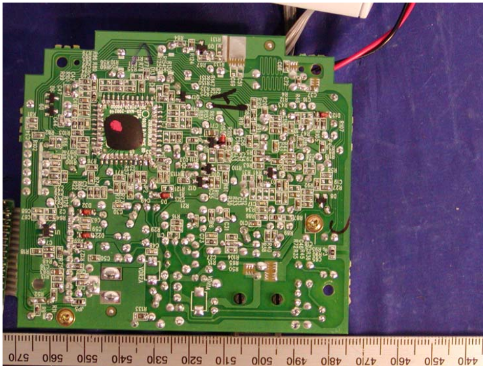
Base Main Board - Solder View (Model: GH3110 & GH3100)
