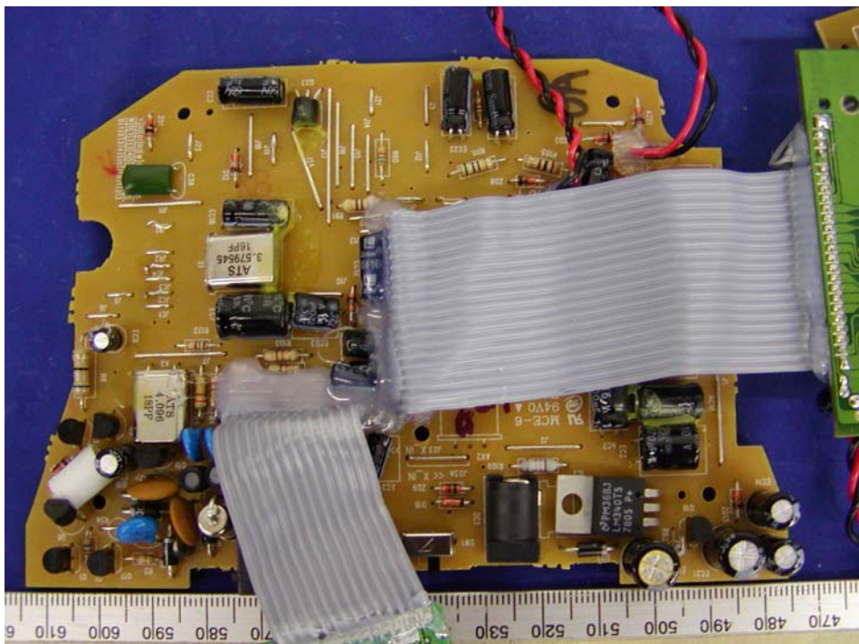
Base - Component View I (Model: GH3150)
