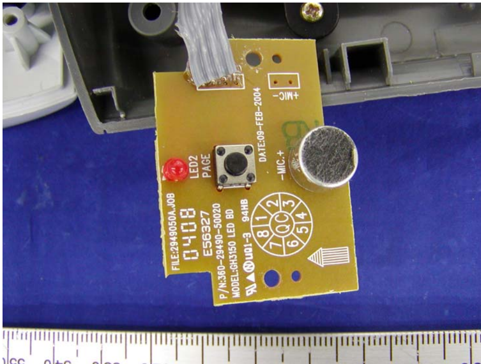
Microphone Board – Component View (Model: GH3150)
