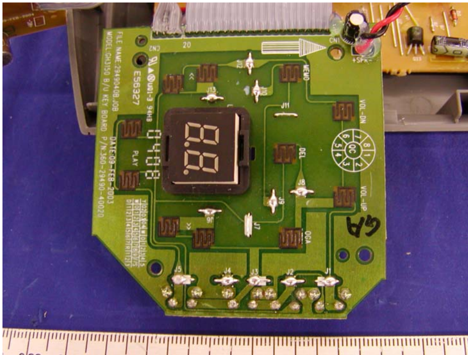
Keyboard - Solder View (Model: GH3150)
