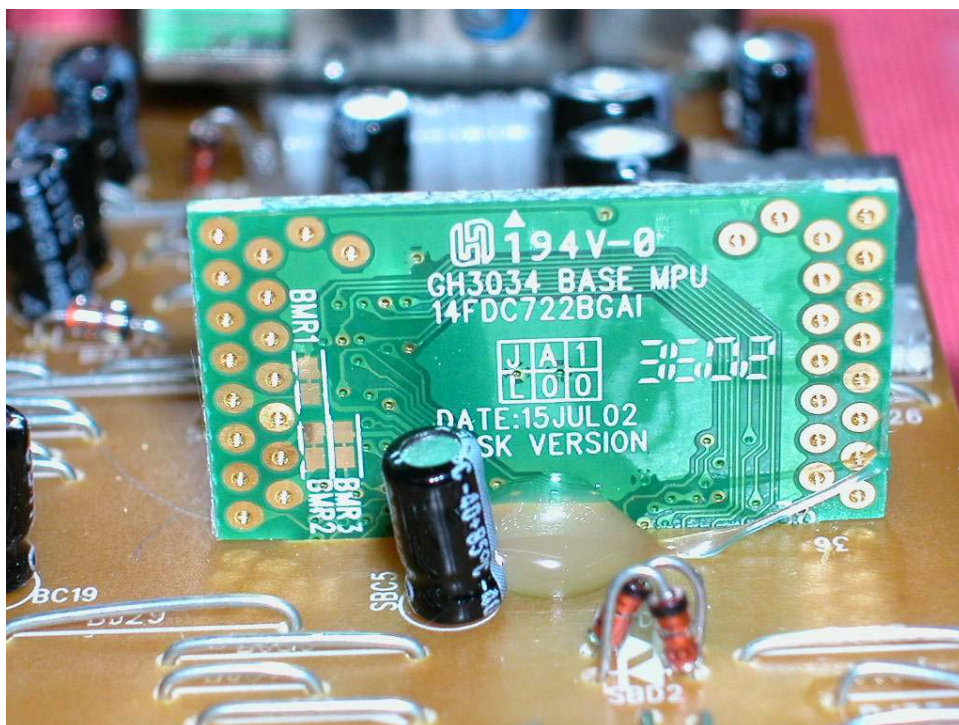
Base Main MPU rear side
