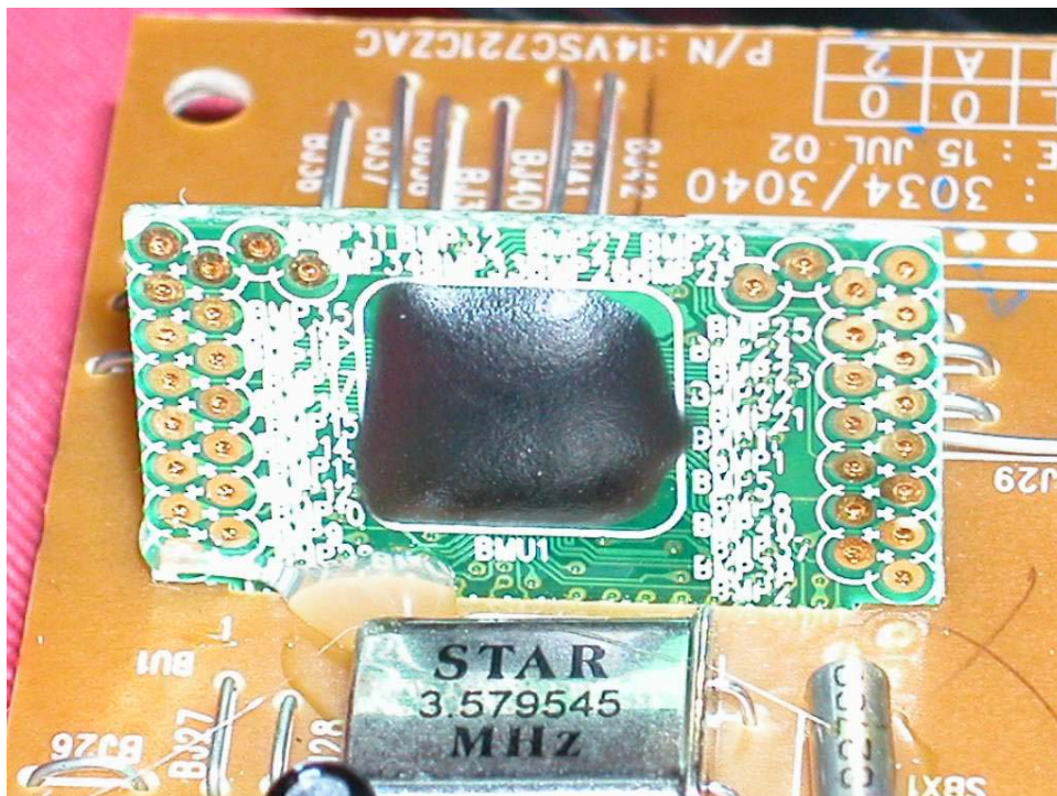
Base Main MPU comp side
