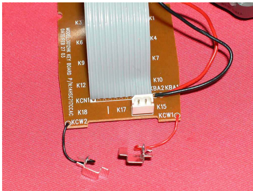
Handset keypad rear side (View 2)
