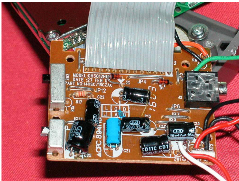
Handset another Main PCB rear side
