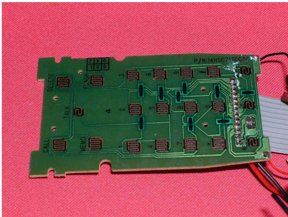
Handset keypad front side
