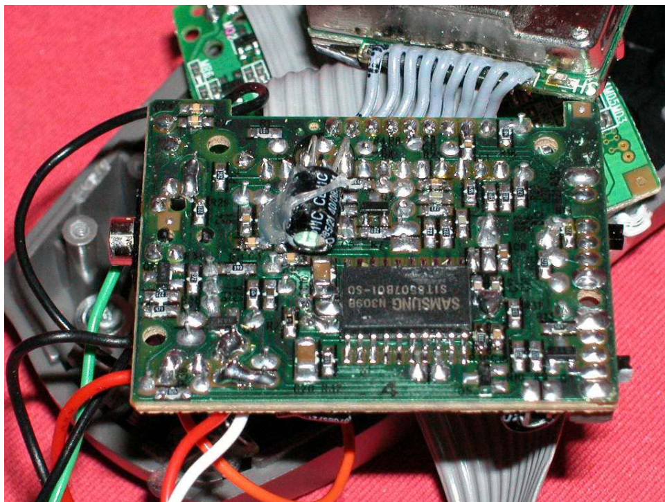
Handset another Main PCB front side
