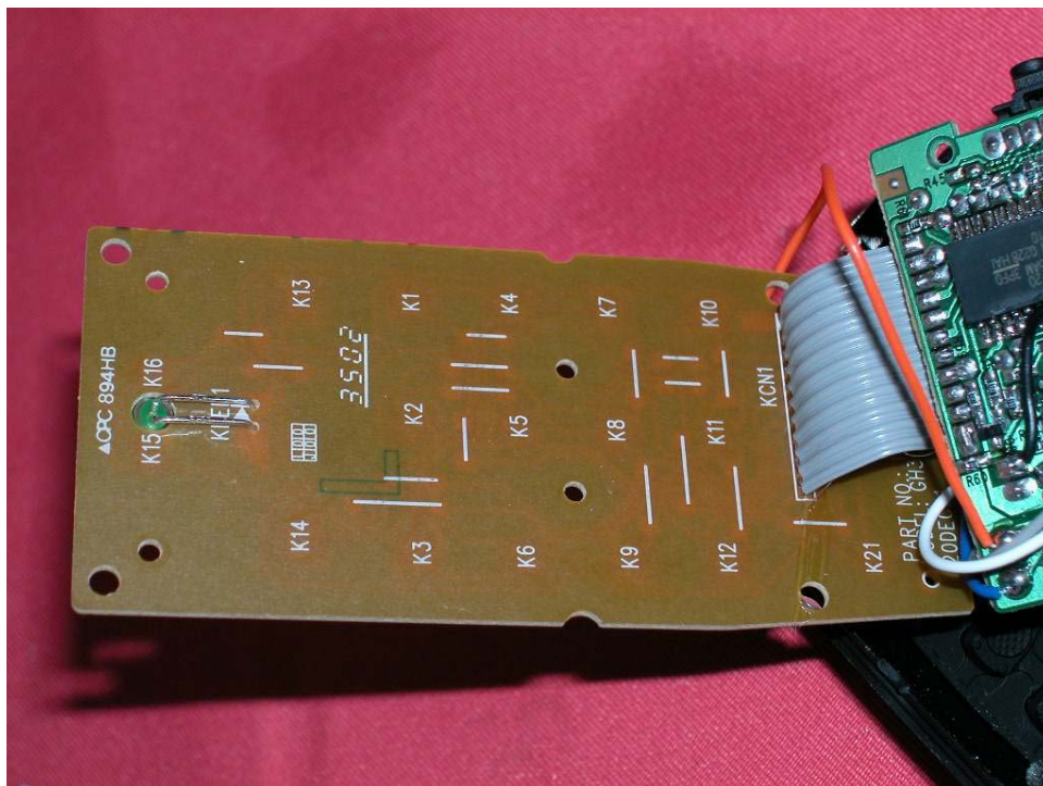
Handset PCB keypad rear side (View 1)
