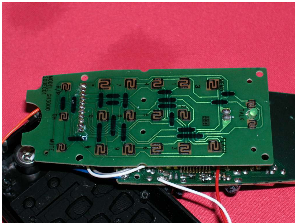
Handset PCB keypad side
