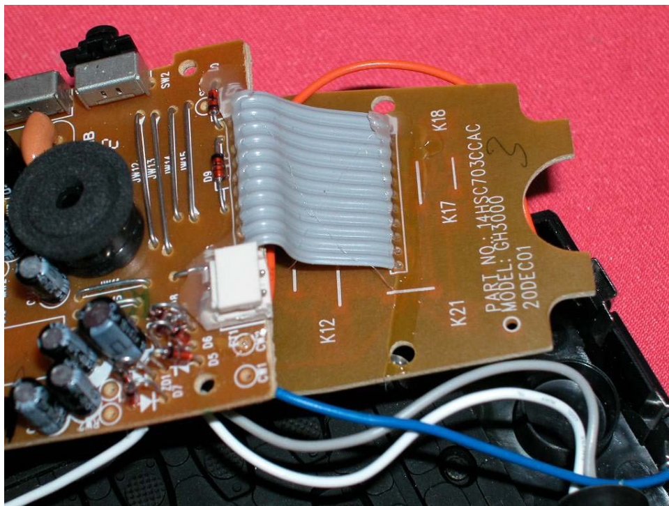
Handset PCB keypad rear side (View 2)
