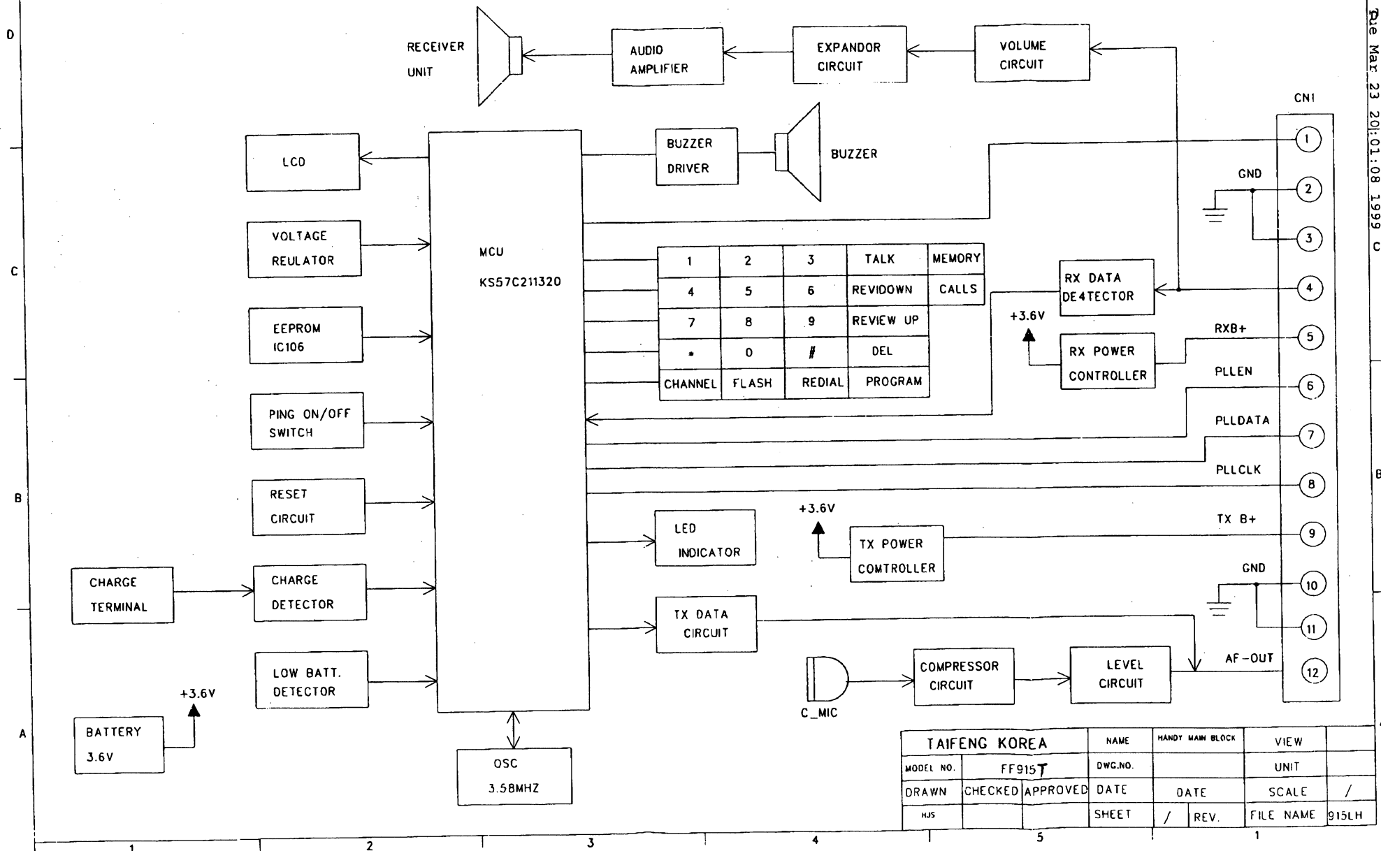
FF915 HAND MAIN BLOCK DIAGRAM
