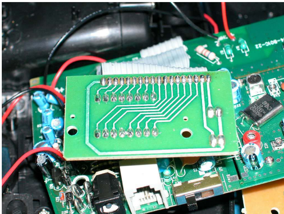
Base LEDs PCB rear side
