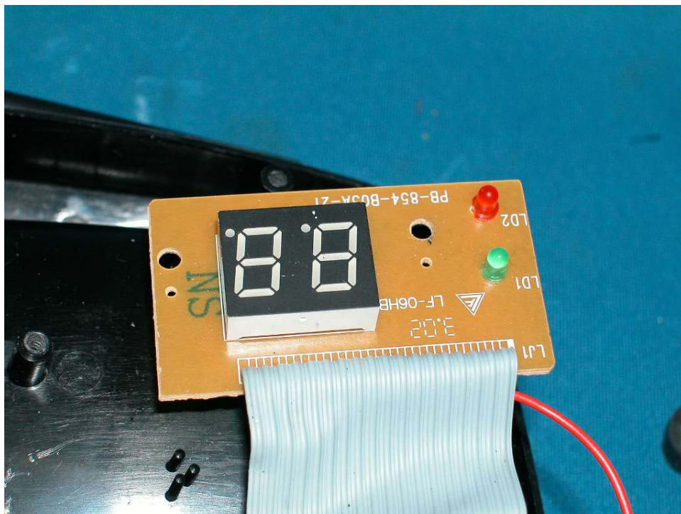
Base LEDs PCB front side
