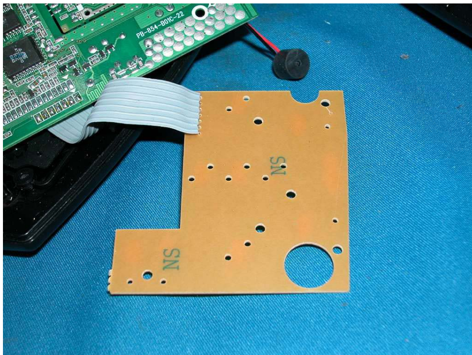
Base DAM keypad rear side
